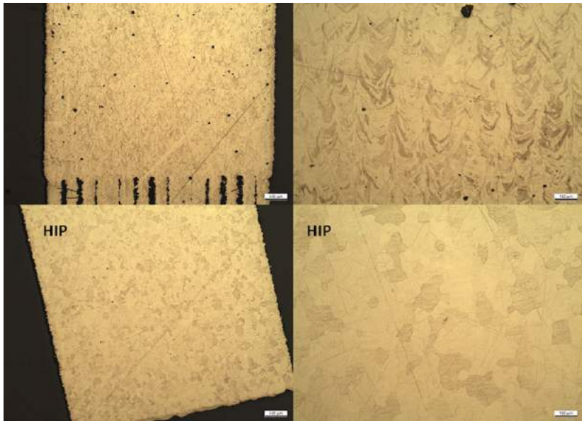
Fig. 11 Vertical cross sections of a Pt950Au PBF-LB sample at different magnifications without and with HIP-treatment
