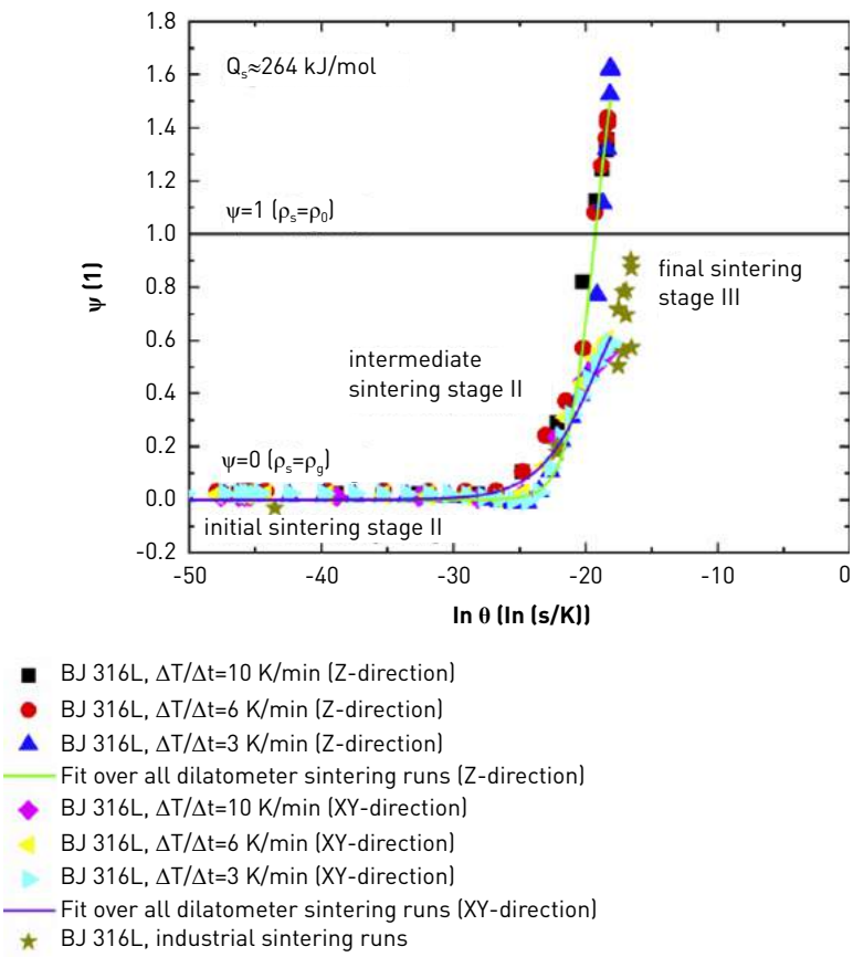
Fig. 3 MSCs of BJ 316L from the different dilatometer sintering runs with n_i=96 data points (the full density of BJ 316L was assumed to be \rho_0=7.93 g/cm 3 to harmonise the current MSC with pycnometer density measurements reported in the literature) [1]
