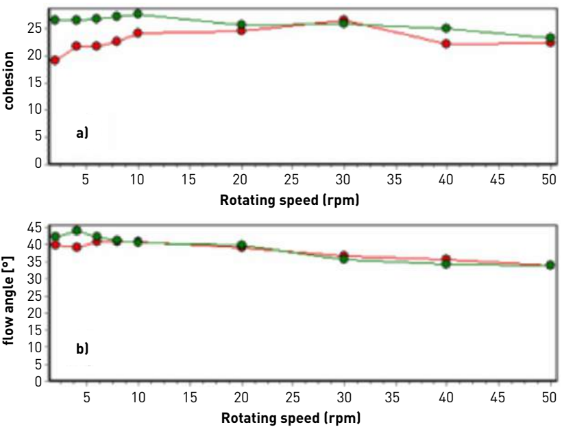
Fig. 4 Powder analysis with GranuDrum: (a) cohesion coefficient, (b) flow angle vs rotating speed [2]
