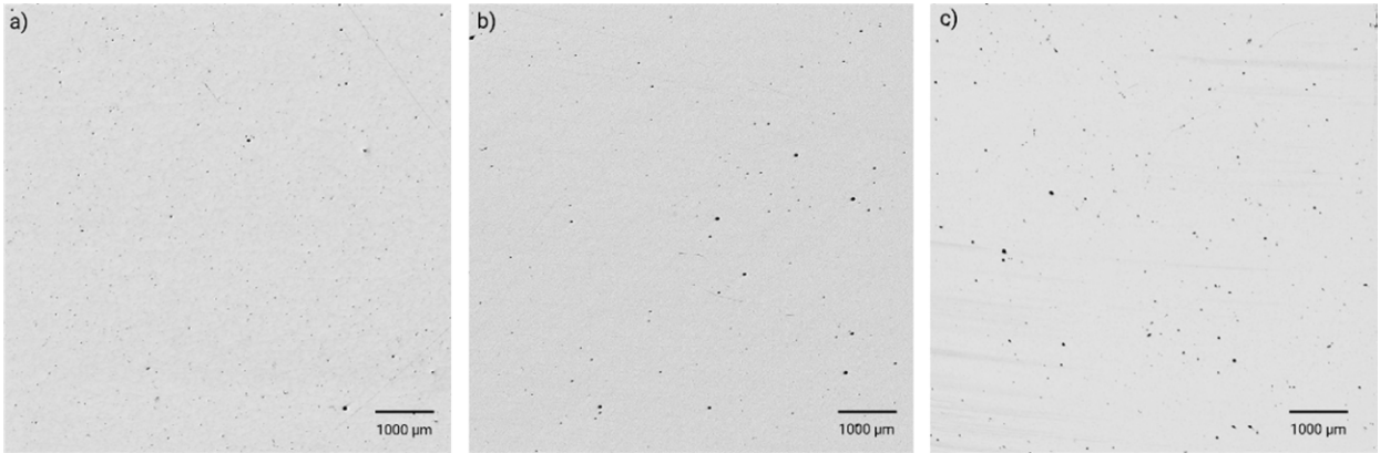
Fig. 4 Optical micrographs with relative densities above 99.85% at (a) 40 cm³/h, (b) 80 cm³/h and (c) 120 cm³/h build speeds
