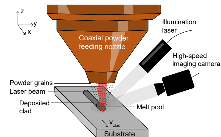
Fig. 1 Schematic illustration of the DED process along with process observation through high-speed imaging
