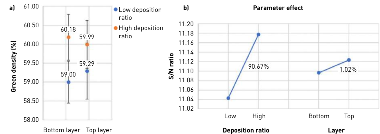
Fig. 7 a) Green density values of the stage 2 experimental trial showing the differences between part location and the amount of material used for powder layer generation; b) parameter effects in green density improvement [2]
