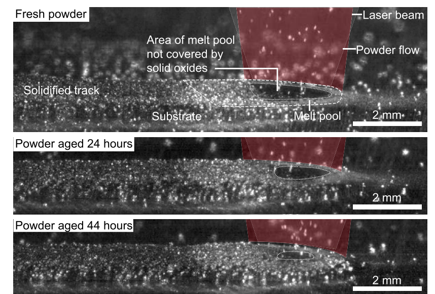
Fig. 4 Frames from high-speed imaging showing the process for fresh and aged powder for the same processing parameters (laser power 6 kW, travel speed 1 m/min and deposition rate 2.75 g/min)
