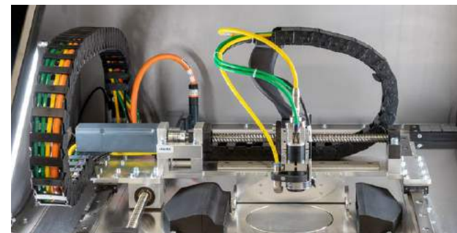
The interior of the Alpha 140 shows the inert gas and axis systems. The spindle-driven axis system allows high positioning and repeatability of the laser system (Courtesy Kurtz Erska)
