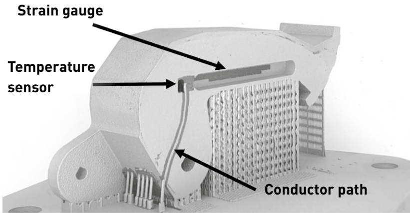
Fig. 5 Demonstrator for a sensor-integrated smart part, built on a modified PBF-LB machine, courtesy Fraunhofer IGC, Augsburg, Germany
