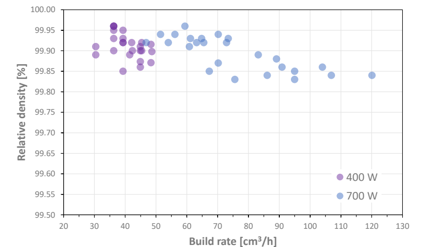
Fig. 3 Monodisperse powders maintain high density across a wide range of build rates and provide a large processing window
