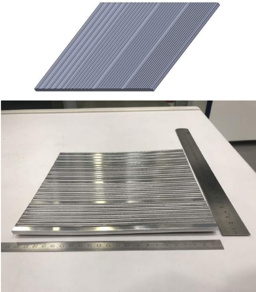
Fig. 6 Stiffening structures potentially used in automotive and railway systems
