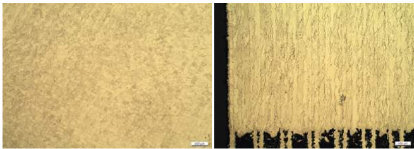
Fig. 10 Microstructure of PBF-LB samples at different high energy inputs
