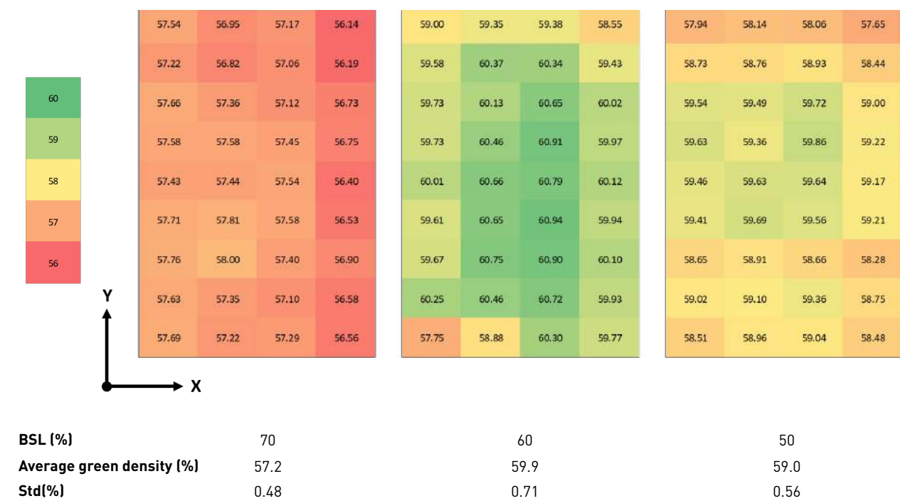
Fig. 6 Green density distribution along the powder bed in Binder Jetting as a function of binder saturation level [2]
