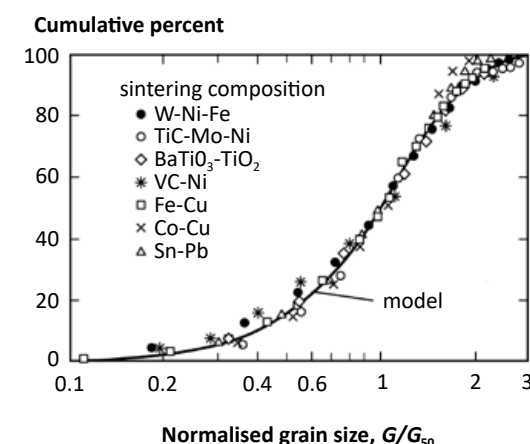
Fig. 15 Cumulative grain size distribution for several sintered materials. The results are compared to a Weibull distribution model where the normalisation factor is the median grain size G_{50} to collapse the results of various studies into a single curve
