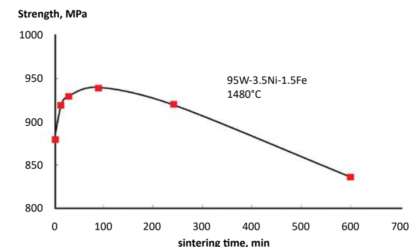
Fig. 6 Over-sintering occurs as materials pass through the peak density and grain size combination. This plot gives tensile strength as a function of sintering time for a tungsten alloy heated to 1480°C in hydrogen for times up to 600 min
