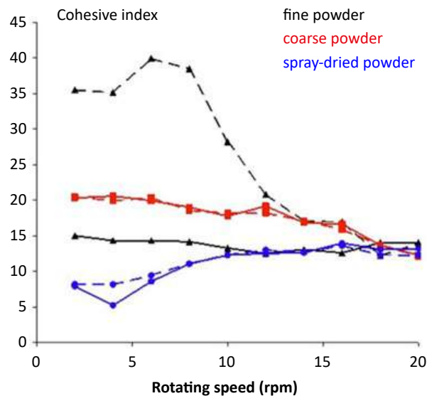
Fig. 7 Cohesive index for fine and coarse powder versus rotating speed [6]
