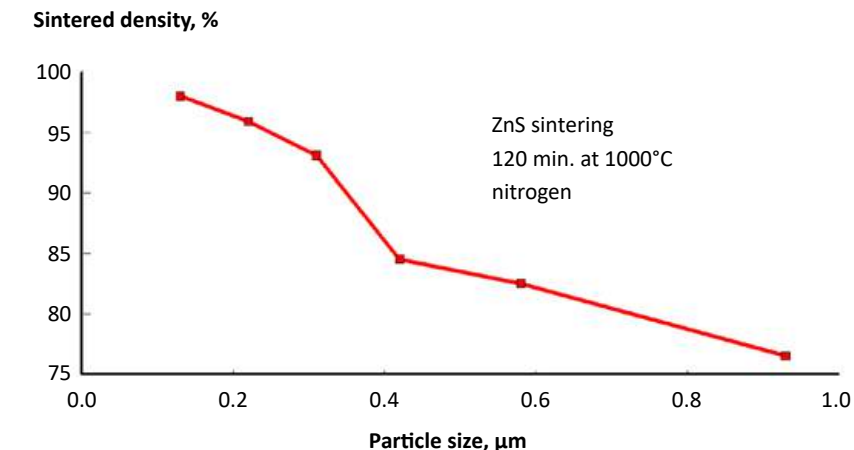
Fig. 5 Sintered density versus particle size for zinc sulfide heated in nitrogen for 120 min. at 1000°C, illustrating the improved densification associated with small powders
