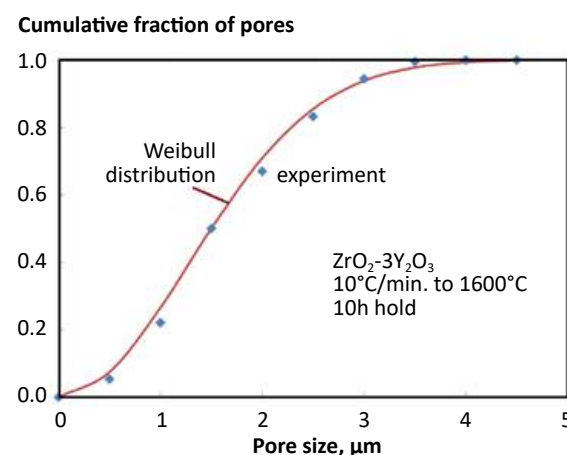
Fig. 17 A demonstration of how the cumulative pore size distribution conforms to a Weibull distribution using data from yttria doped zirconia sintered at 1600°C
