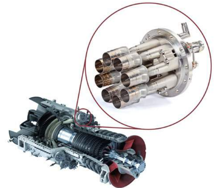
Fig. 1 Swirlers and burner assembly and their location in the gas turbine (Courtesy Siemens)
