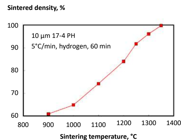
Fig. 18 Plot of sintered density versus peak temperature for 10 μm 17-4 PH stainless steel
