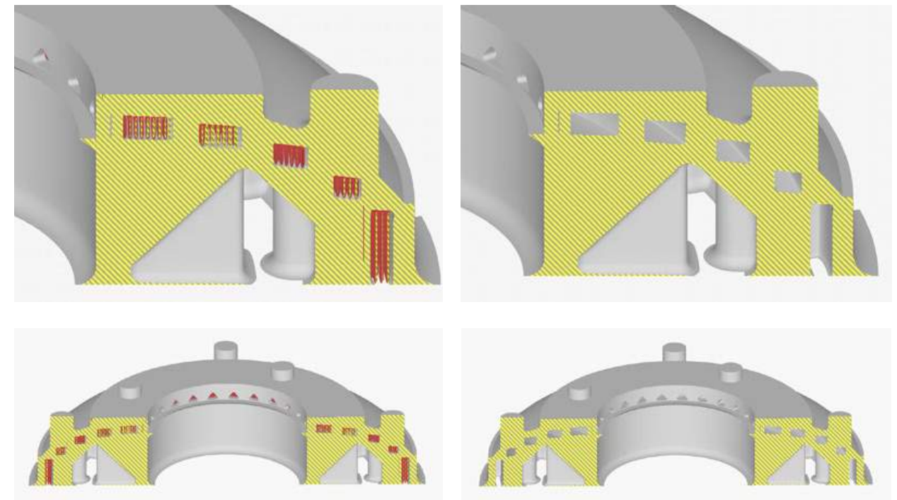
Fig. 7 Cross section overview and details showing support structures within the channels (left) if the diffuser housing were to be printed by existing L-PBF platforms, versus how the Velo3D Sapphire system can print the channels support-free. Machining the support structures in this specific part design would be incredibly complex.
