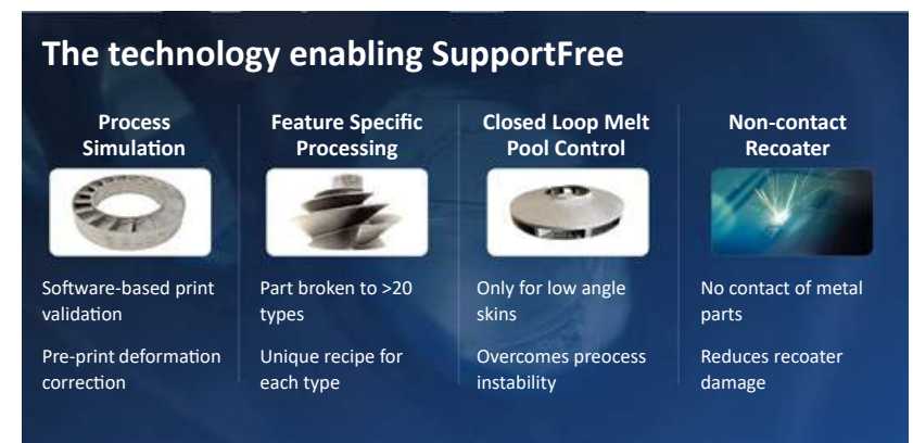
Fig. 4 This is the foundation to Velo3D's SupportFree technology, which is a combination of simulation from Flow, in-process metrology, and its non-contact recoater
