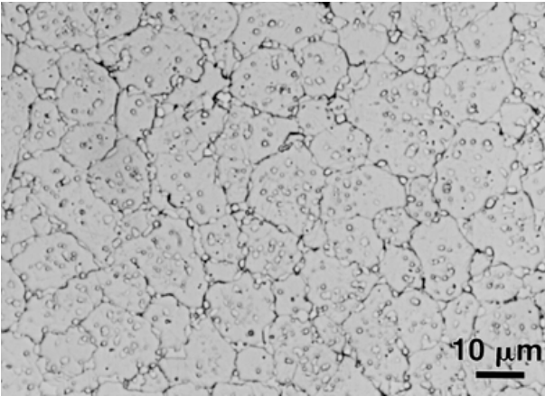
Fig. 9 Microstructure after supersolidus liquid phase sintering a M2 tool steel containing 0.8% carbon. The powder densifies in 10 min. at 1280°C using a nitrogen-hydrogen atmosphere
