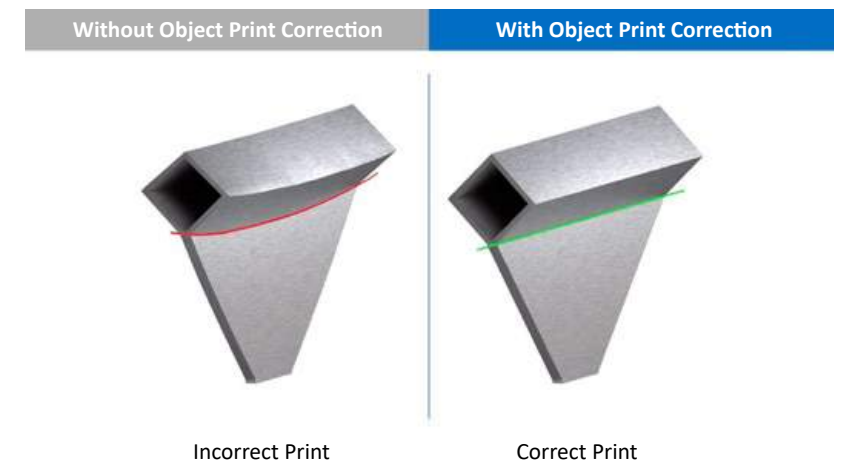
Fig. 3 Object Print Correction (OPC) within Velo3D's Flow software corrects build deformation issues before the build begins. The simulation engine applies counter-deformation to the part to ensure that the first build is a good build
