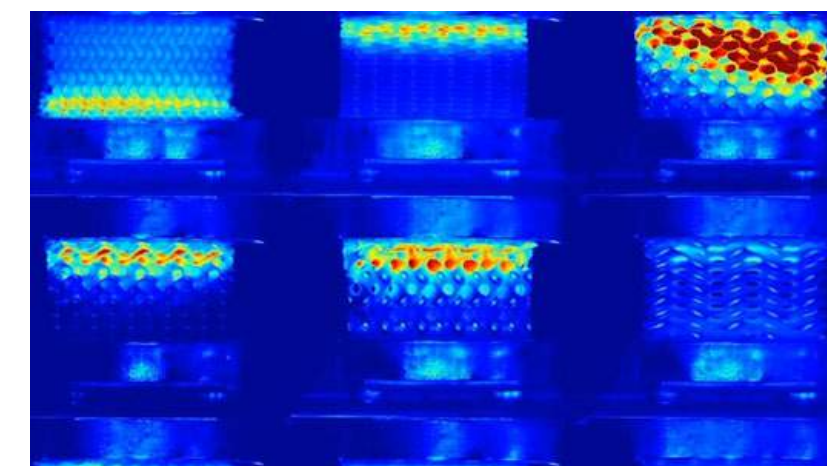
Thermal imagery of parts additively manufactured with AF-9628 powder. (Courtesy photo/Air Force Institute of Technology)
