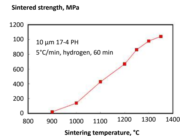
Fig. 19 Sintered tensile strength for 17-4 PH stainless steel heated at 5°C/min. with a 60 min. hold at various peak temperatures
