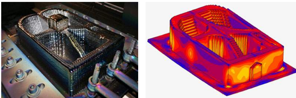
Fig. 3 A photo of a complex AM part (left) and a simulation showing the predicted residual stress (Courtesy of Vu Nguyen)
