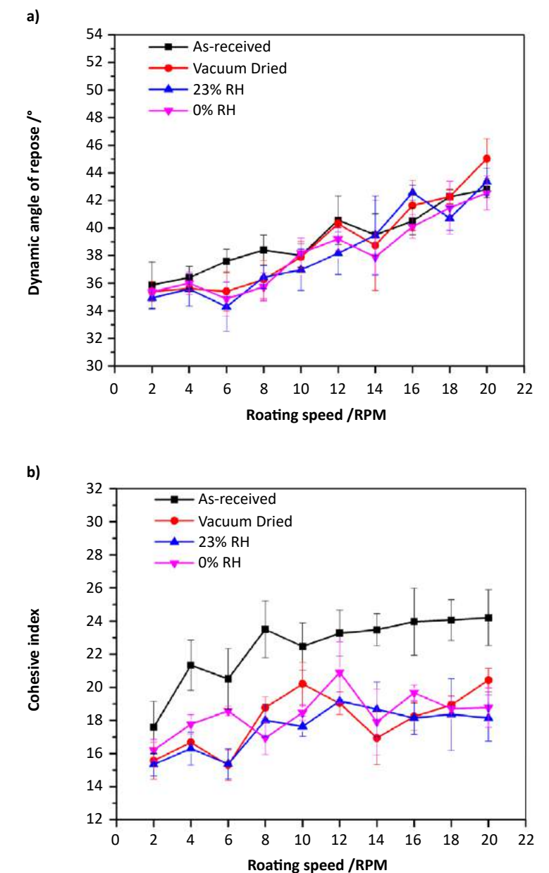
Fig. 8 The evolution of the dynamic angle of repose (a) and cohesive index (b) as a function of the rotating speed for IN625 in different states: the initial powder as-received, after exposure in a container for 90 days, vacuum dried at 200°C for 1 h, the dried powder exposed in relative humidity of 23% and the dried powder stored in a container at 0%RH [4]
