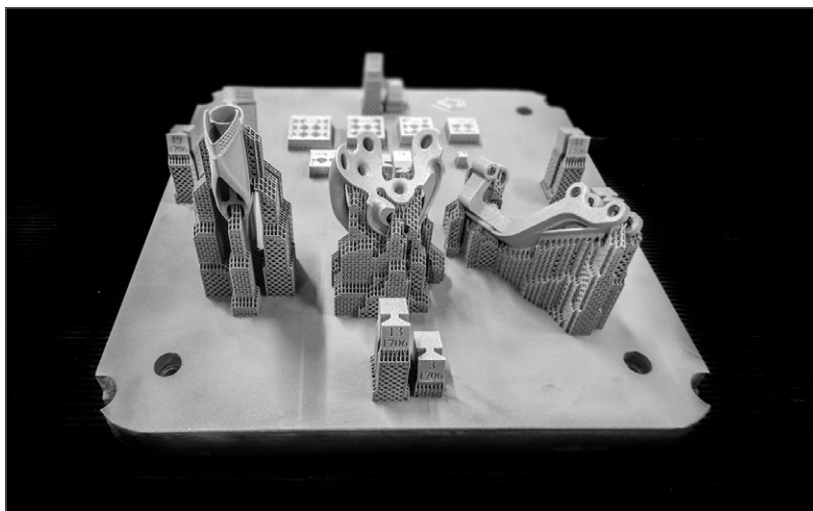
Fig. 9 Metal additively manufactured parts with support structures generated in Materialise Magics
