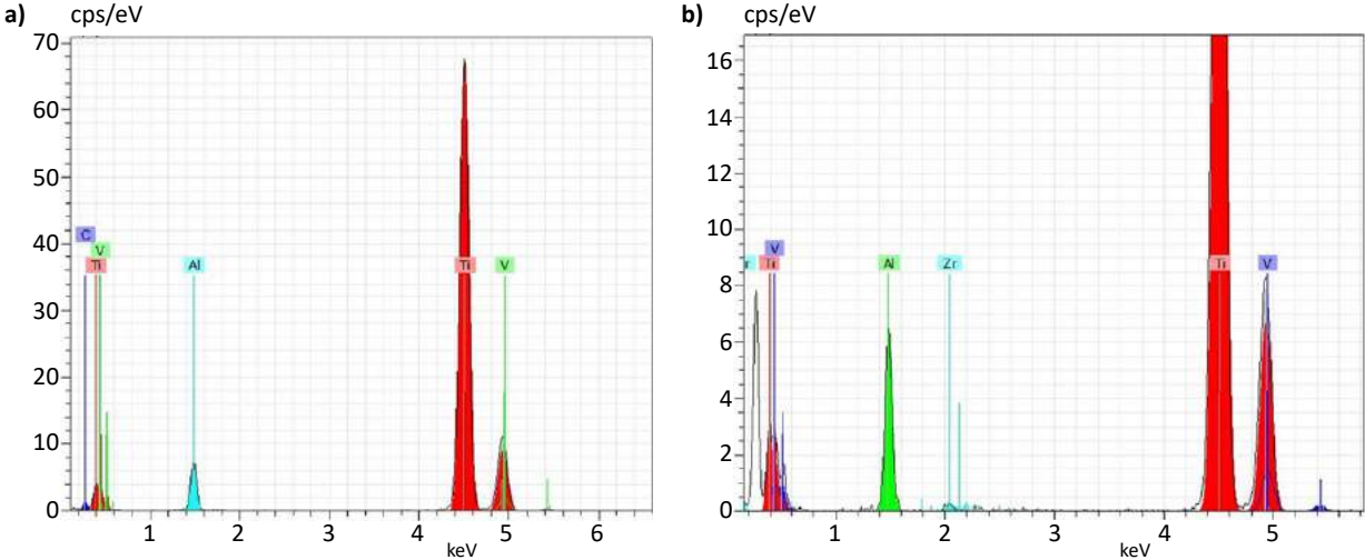
Fig. 4 Representative EDS spectra for the Ti64_MS1 (a) and Ti64_ZrO 2 (b) samples [2]
