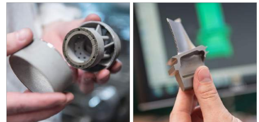
Additively manufactured gas turbine burner head (left) and gas turbine blade (right) for use in power plant operation
