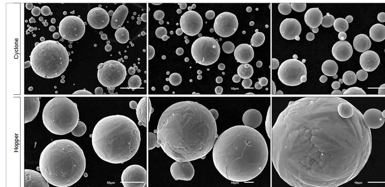
Fig. 4 SEM image of spheroidal Cristal Metals Ti metal powder AR3-20170609.02 [Courtesy Cristal Metals]
