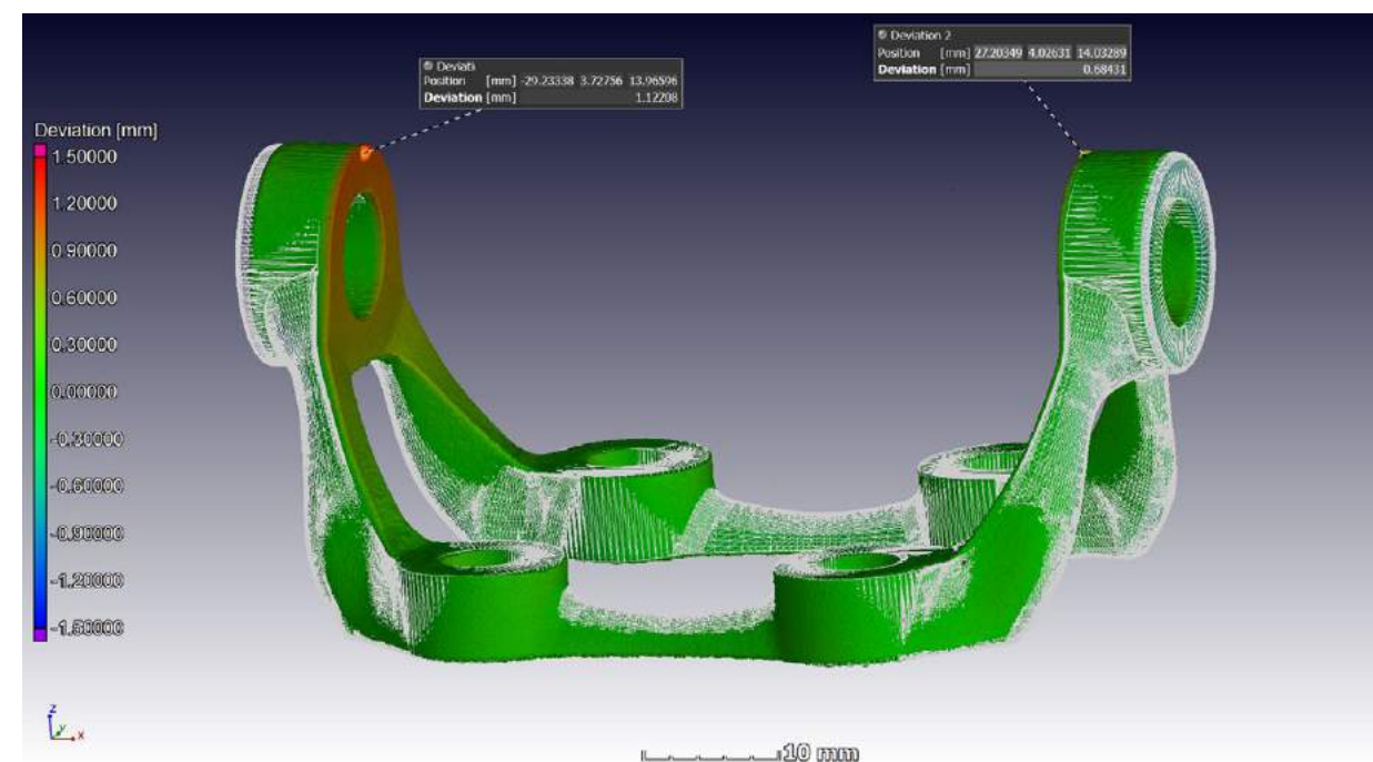
Fig. 5 Example of bracket warping – CAD variance more than 1 mm (CAD file shown in wireframe, actual part with colour coded variance)
