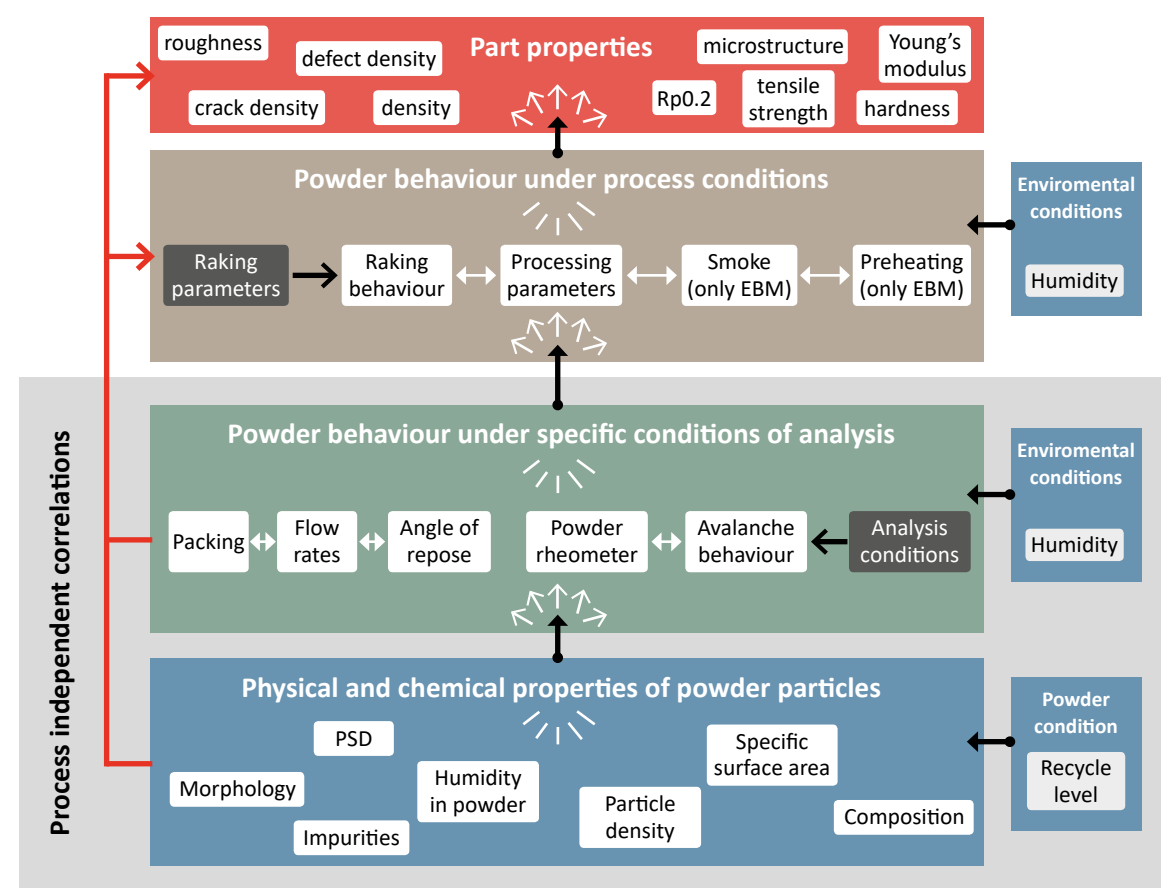
Fig. 5 Schematic of the database, capable of tracking the influence of powder along the PBAM process chain [3]
