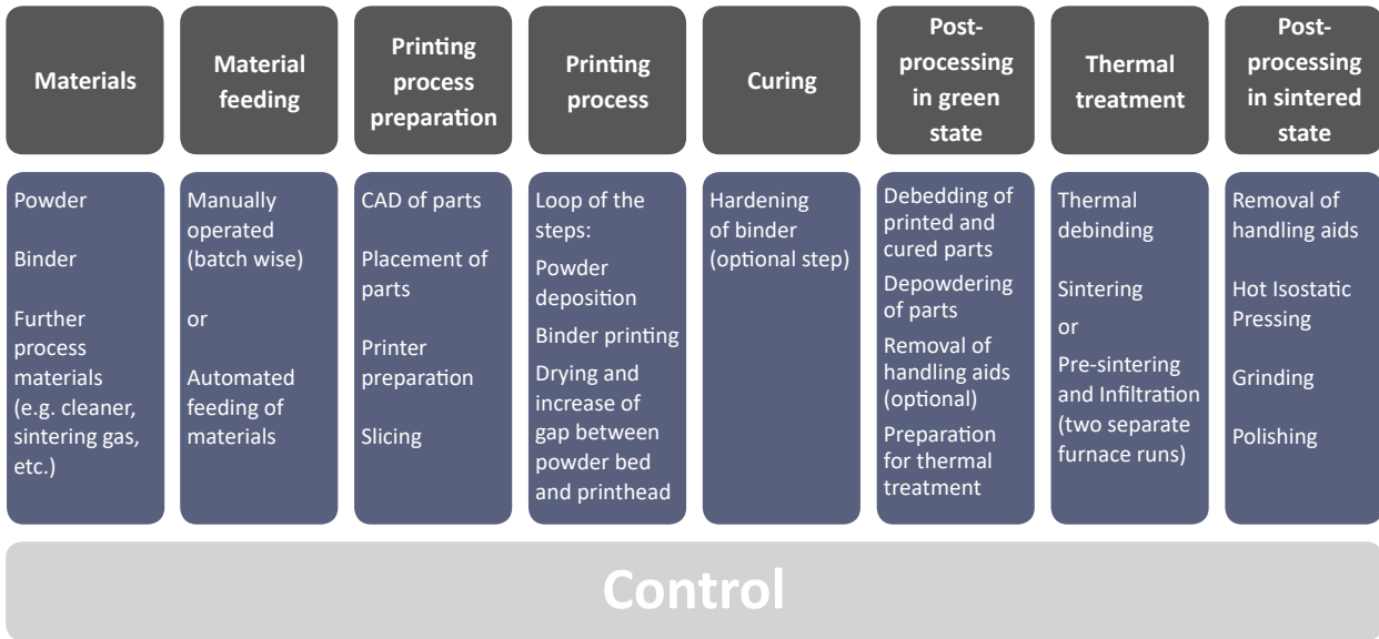
Fig. 3 Overview of all process steps in the Binder Jetting process
