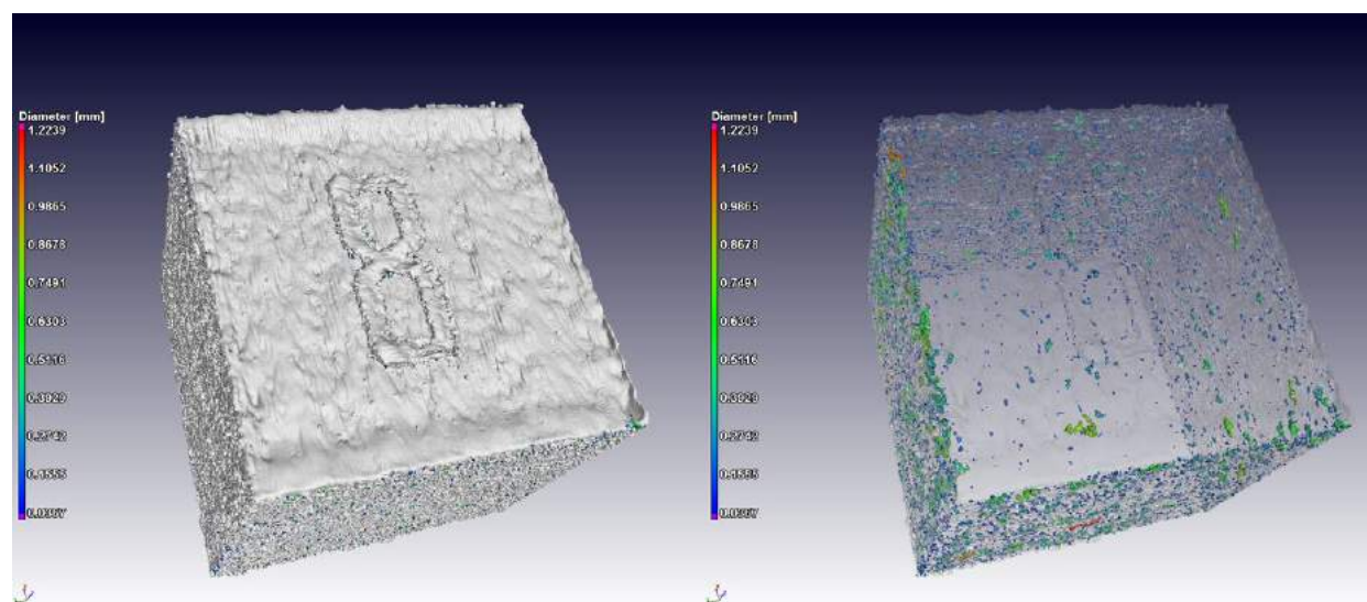
Fig. 3 Coupon cube sample showing porosity mainly around the edges, attributed to contour scanning error. Laser-Beam Powder Bed Fusion sample of Ti-6Al-4V, using standard method [20]. Pores are colour coded by diameter, the front facing surface with number 8 is the top surface of the cube – this shows the pores are mostly located around the vertical cube edges
