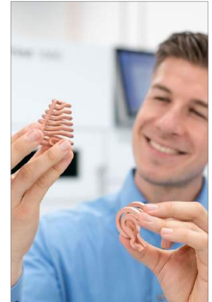
Using a green laser connected to its TruPrint 1000 metal AM machine, Trumpf has been able to additively manufacture pure copper and gold components
