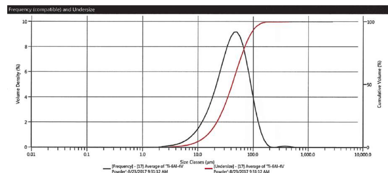
Fig. 6 A typical distribution of Ti-6Al-4V produced by Cristal Metals and Arcast
