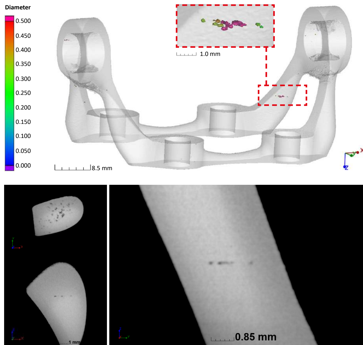
Fig. 6 Layered flaw found in complex part shown here in multiple microCT views
