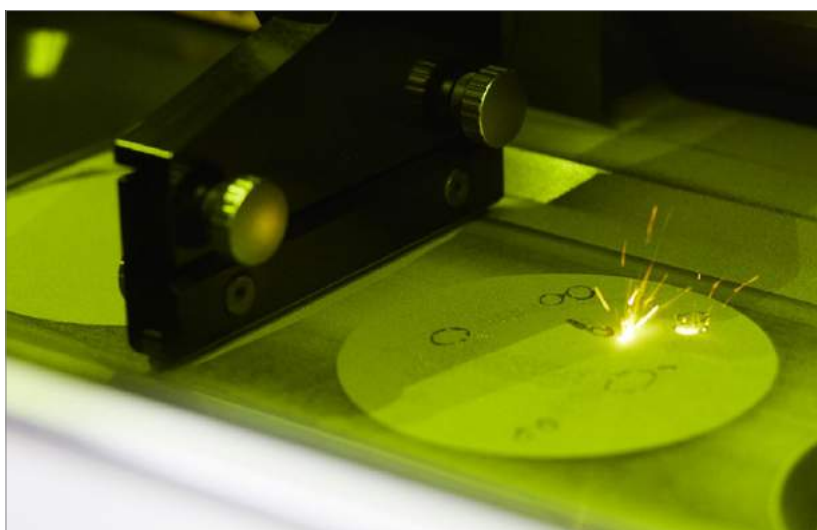
A view of the build chamber during component manufacture on Trumpf's TruPrint 1000
