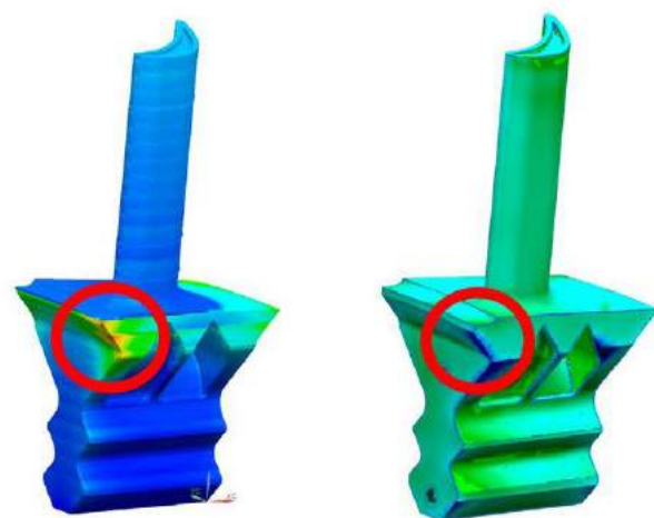
Fig. 7 Siemens' Simcenter 3D AM Process Simulation tool shows how the predicted distortion (on the left) is confirmed by the comparison of the real-world part to the original CAD data on the right
