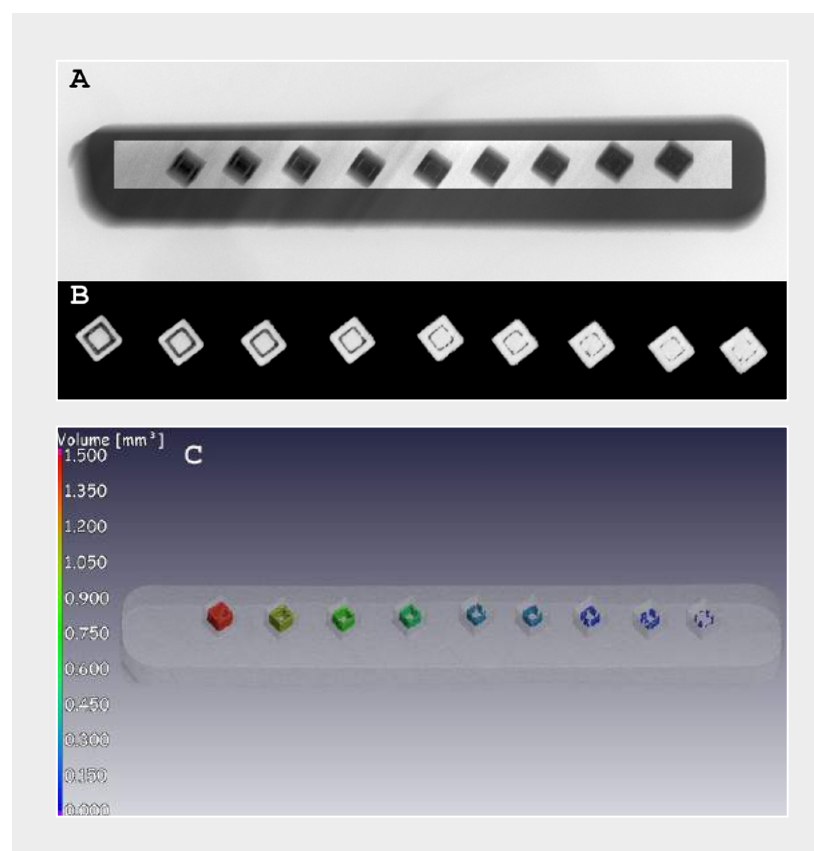
Fig. 2 Intentionally-designed cavities in a Ti-6Al-4V test part, produced by Laser-Beam Powder Bed Fusion, taken from [26]. Shown here are (A) an X-ray projection image with region contrast enhanced, (B) a microCT scan slice image in horizontal plane and (C) a 3D rendering including porosity/defect analysis showing cavities colour-coded by volume
