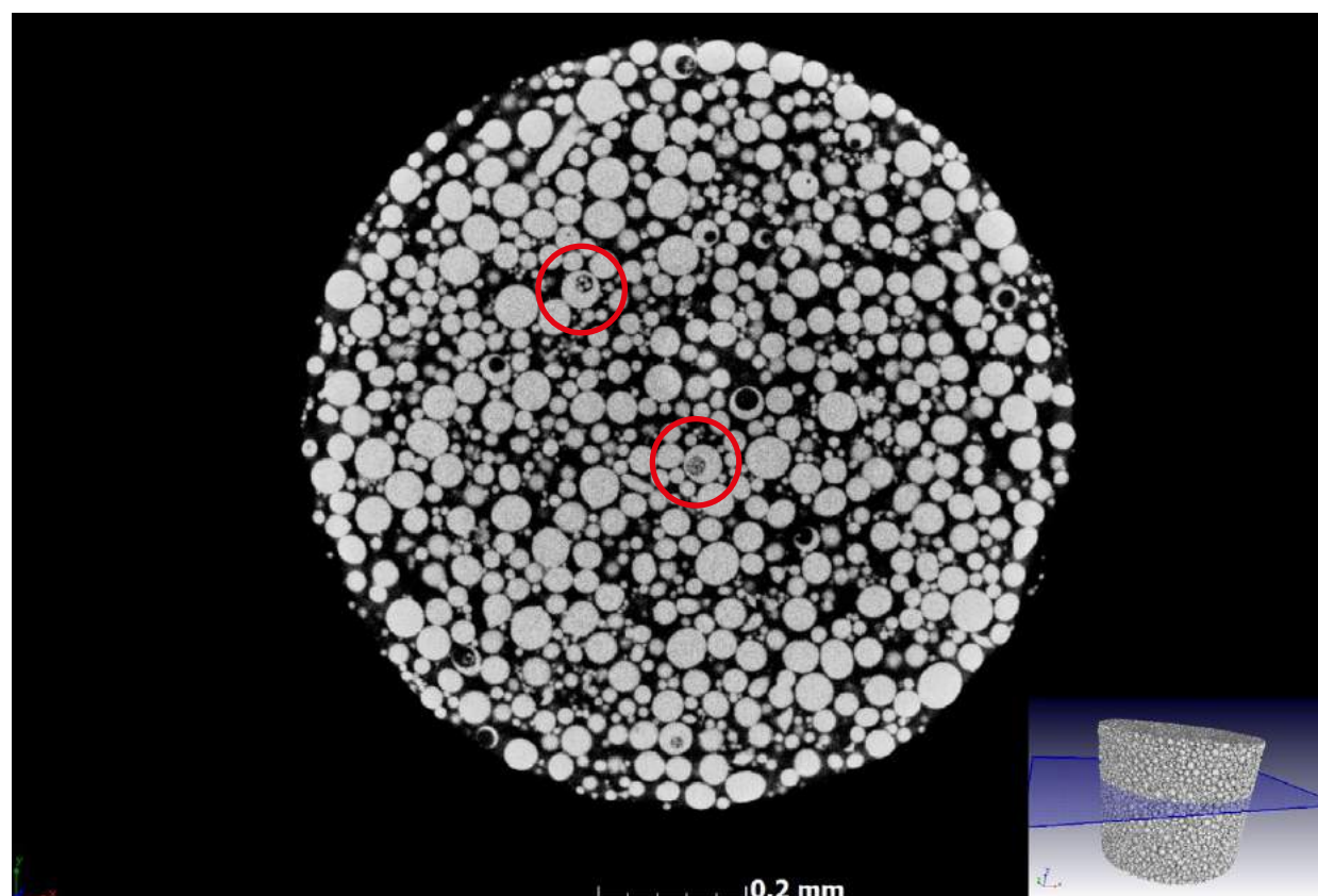
Fig. 8 Powder analysis showing a typical cross sectional view of gas atomised Ti-6Al-4V powder. The red circles show powder particles which contain pores filled with finer powder particles
