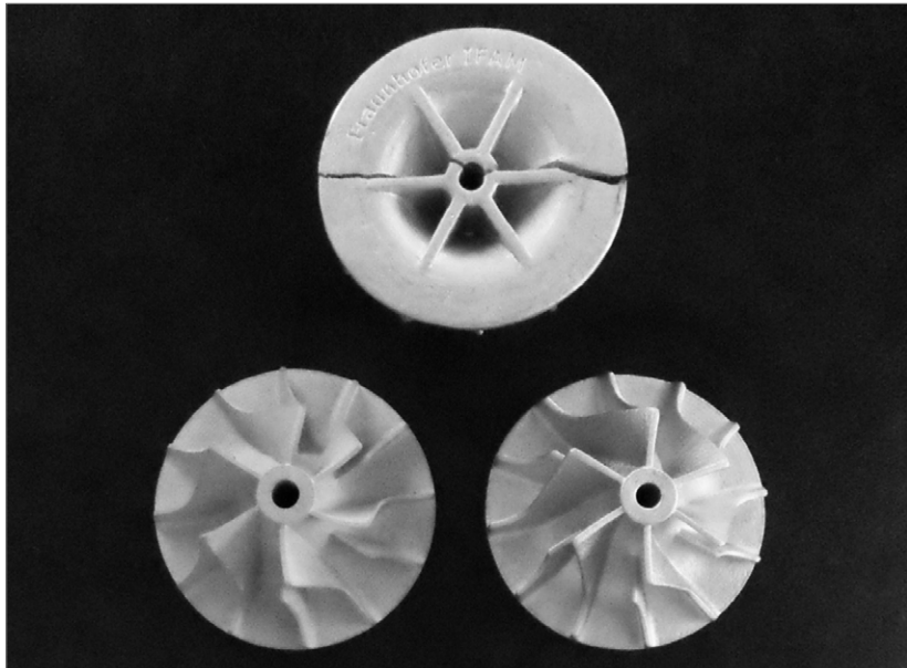
Fig. 2 Turbine wheels made by binder jetting, upper part broken due to high cooling rates after sintering; lower left part with significant distortion; lower right part with less distortion
