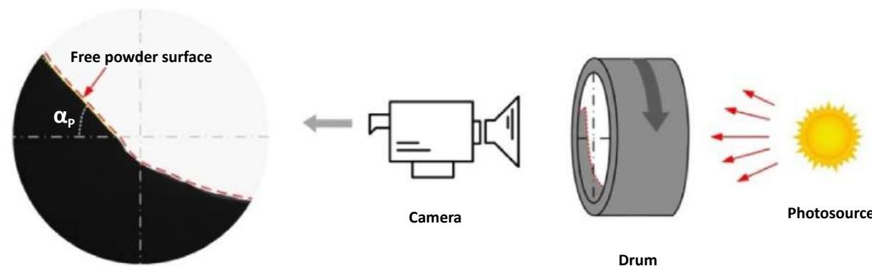
Fig. 7 Schematic of the GranuDrum™ technique [4]
