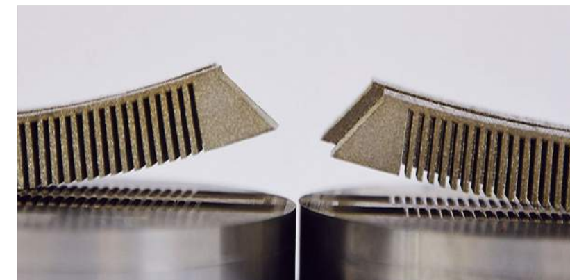
The component preheated with VCSEL (right) has significantly less distortion than the component not preheated for the exposure process
