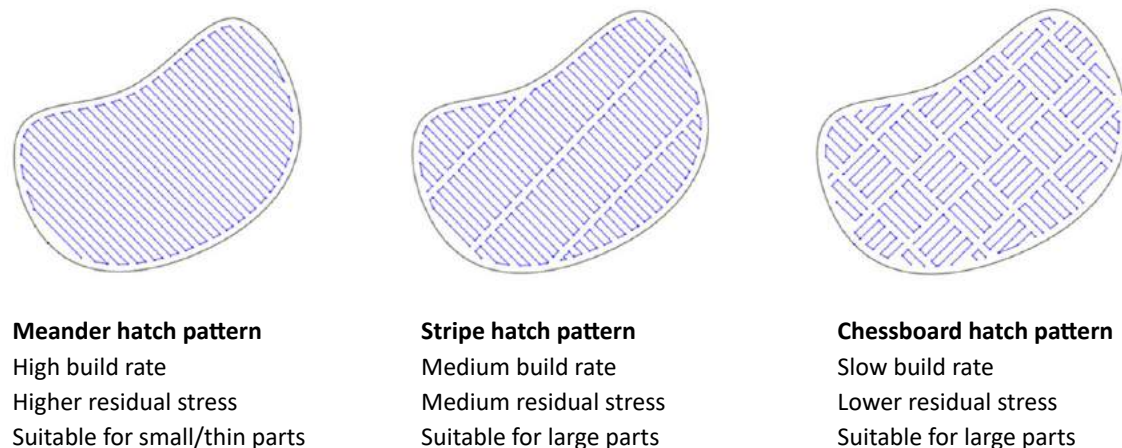
Fig. 3 Laser scan strategies for reducing residual stress
