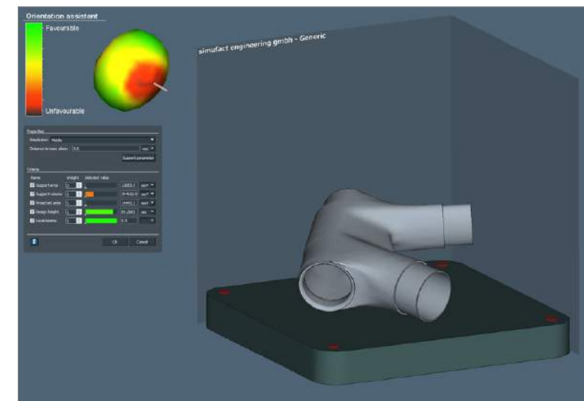
Fig. 8 Simufact Additive 4's orientation assistant helps to determine the best build orientation
