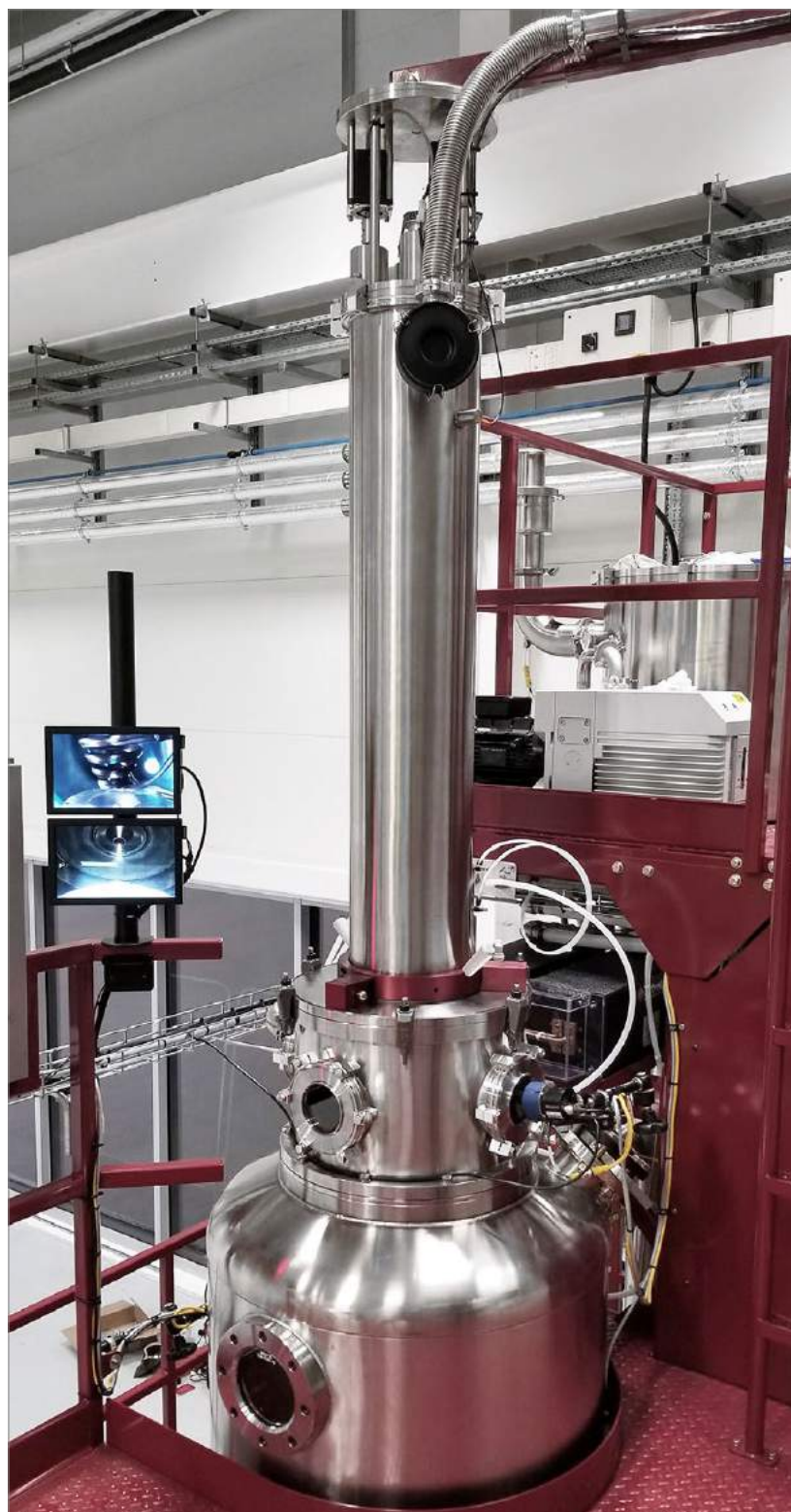
Fig. 5 Detail view of an Arcast inert gas atomiser
