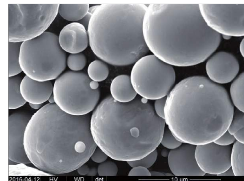
Fig. 7 Steel alloy powders produced using Arcast technology
