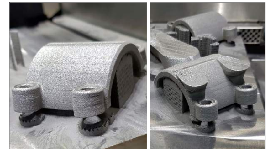
Fig. 1 Examples of parts detaching from the build due to residual stress (Courtesy Alexander Liu)
