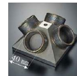
Examples of dot forming technology (Courtesy Mitsubishi Electric)
