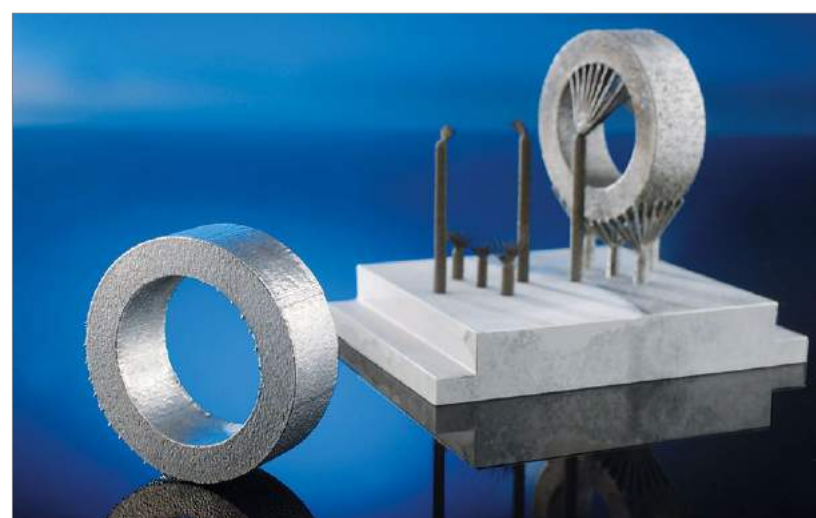
A test piece with supports removed through a wet-chemical process (Courtesy Fraunhofer ILT)
