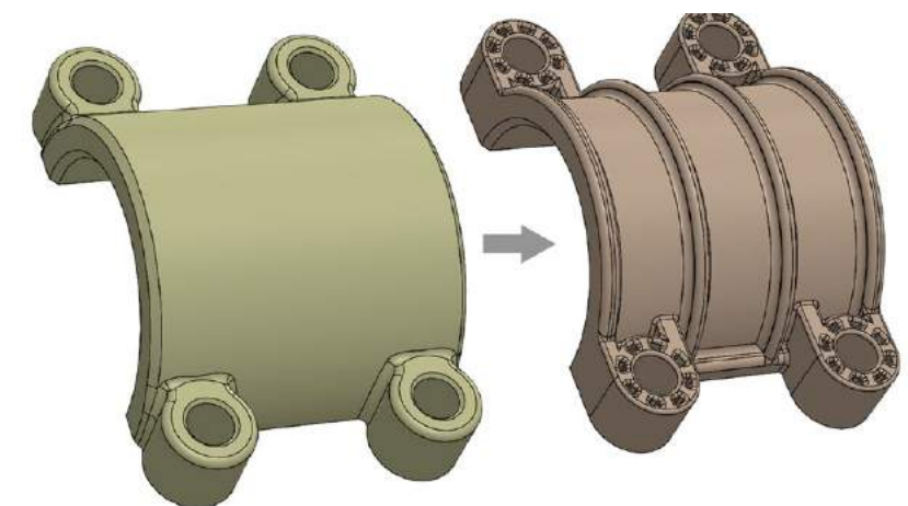
Fig. 5 The original design (left) and new design (right). The new design has an even wall thickness and no areas where stress can build up. It also weighs 25% less
