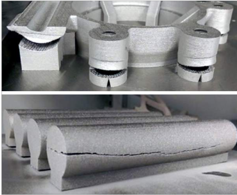
Fig. 2 Examples of the catastrophic effect residual stress can have on parts (Courtesy Renishaw)
