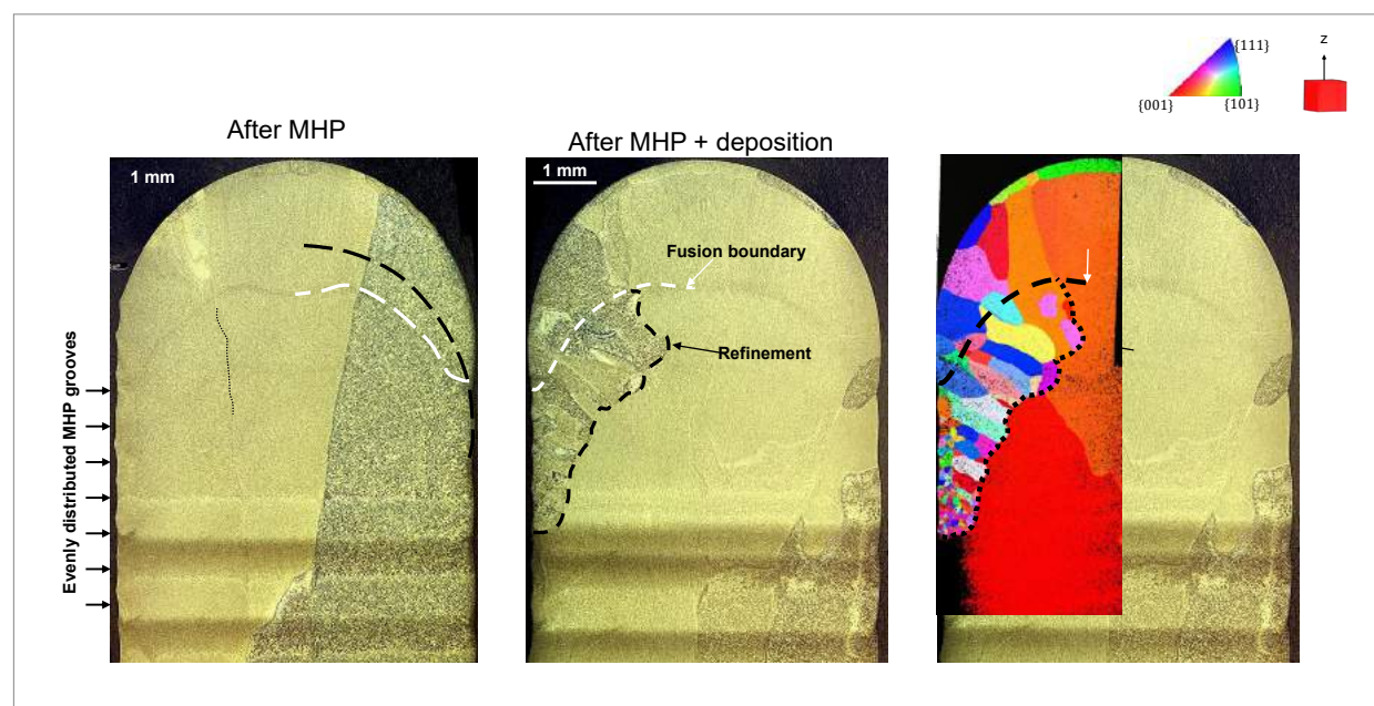
Fig. 6 Jan Roman Hönnige, Cranfield University, UK discussed spatially tailored mechanical properties in Ti-6Al-4V wire-arc additively manufactured components. The tailoring of mechanical properties was achieved by rolling and, in a second approach, machine hammer peening to increase surface hardness
