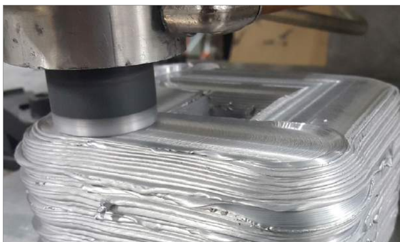
MELD is a solid-state process which can use a wide range of materials as feedstock, including metal powders and rods
