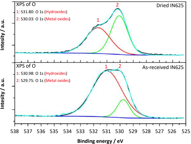
Fig. 9 XPS results of the oxygen binding energies for as received and dried IN625 [4]
