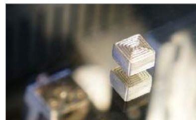
Hardmetal sample with a complex geometry produced on a standard FFF AM system
