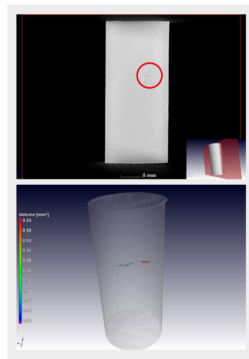
Fig. 7 Witness specimen analysis of quality of build, showing a layered stop-start flaw in this case
