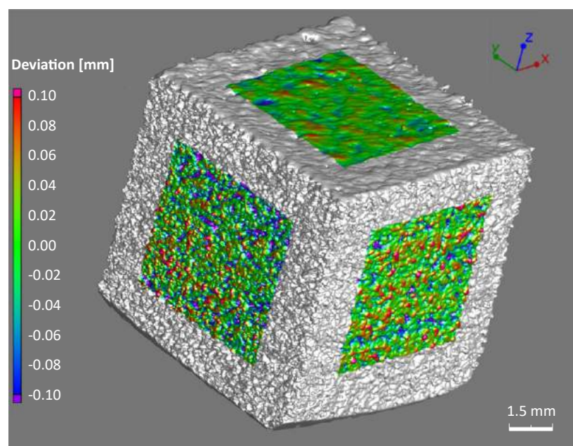
Fig. 4 Surface roughness using microCT, showing three surfaces with colour-maps indicating the top surface is much smoother
