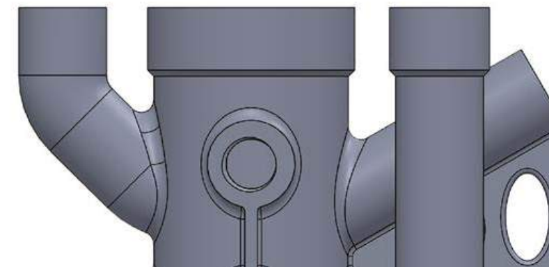
Fig. 10 Material was added to the pipes for subsequent tapping of screw threads, with a 45° chamfer to eliminate the need for support material
