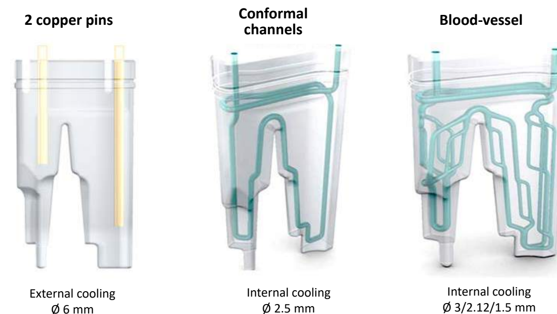
Fig. 6 Possible cooling concepts for an injection moulding tool insert (Courtesy University of Leoben)
