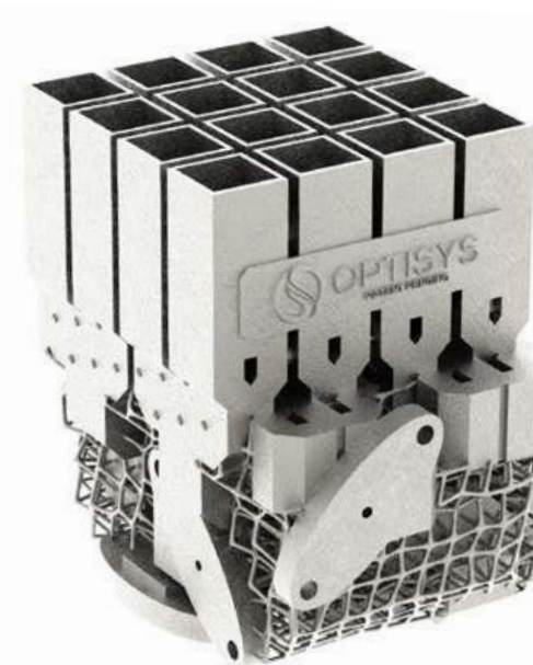
Fig. 3 Optisys designed and manufactured the one-piece, functional assembly antenna shown on the left by optimising a 100-piece design for AM. As shown on the right, high-frequency electromagnetic field simulations are used to analyse and optimise AM antenna designs for maximum RF performance
