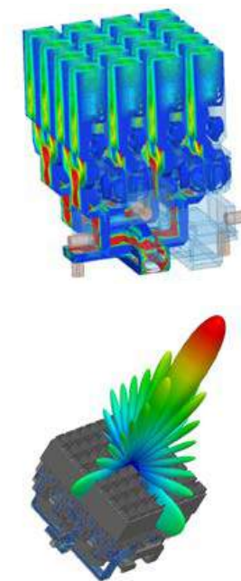
Fig. 3 Optisys designed and manufactured the one-piece, functional assembly antenna shown on the left by optimising a 100-piece design for AM. As shown on the right, high-frequency electromagnetic field simulations are used to analyse and optimise AM antenna designs for maximum RF performance
