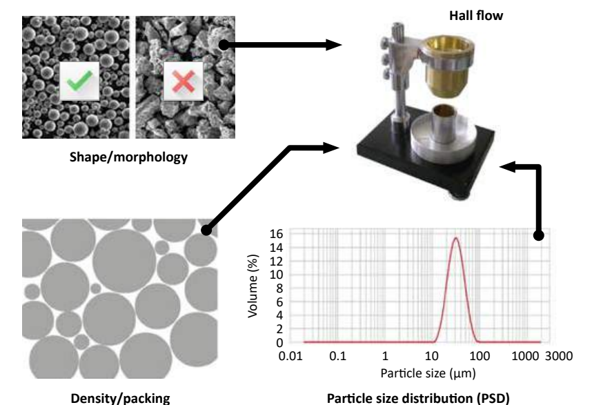
Fig. 1 Important physical properties of metal powders for AM include shape/morphology, particle size distribution (PSD), density/packing and flow [1]
