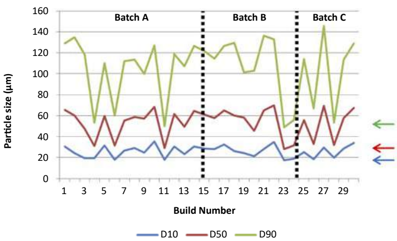
Fig. 12 Variation in particle size – Position 2 [2]
