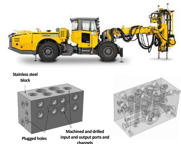
Fig. 1 Top, an Atlas Copco underground drilling rig and bottom, the company's original manifold block design
