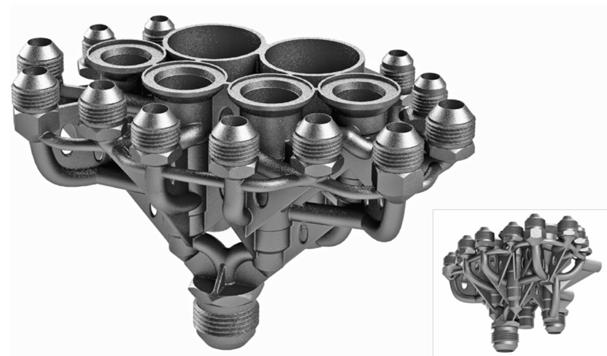
Fig. 4 Top and bottom views of the finished optimised stainless steel AM hydraulic manifold
