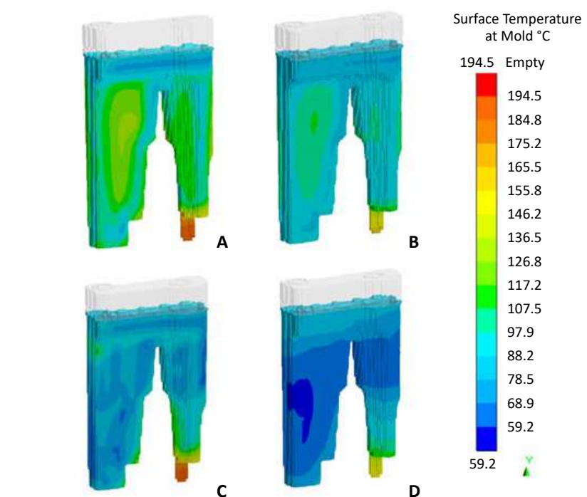
Fig. 7 Surface temperature of the mould insert 3.5 s after the start of the moulding cycle (Courtesy University of Leoben)
