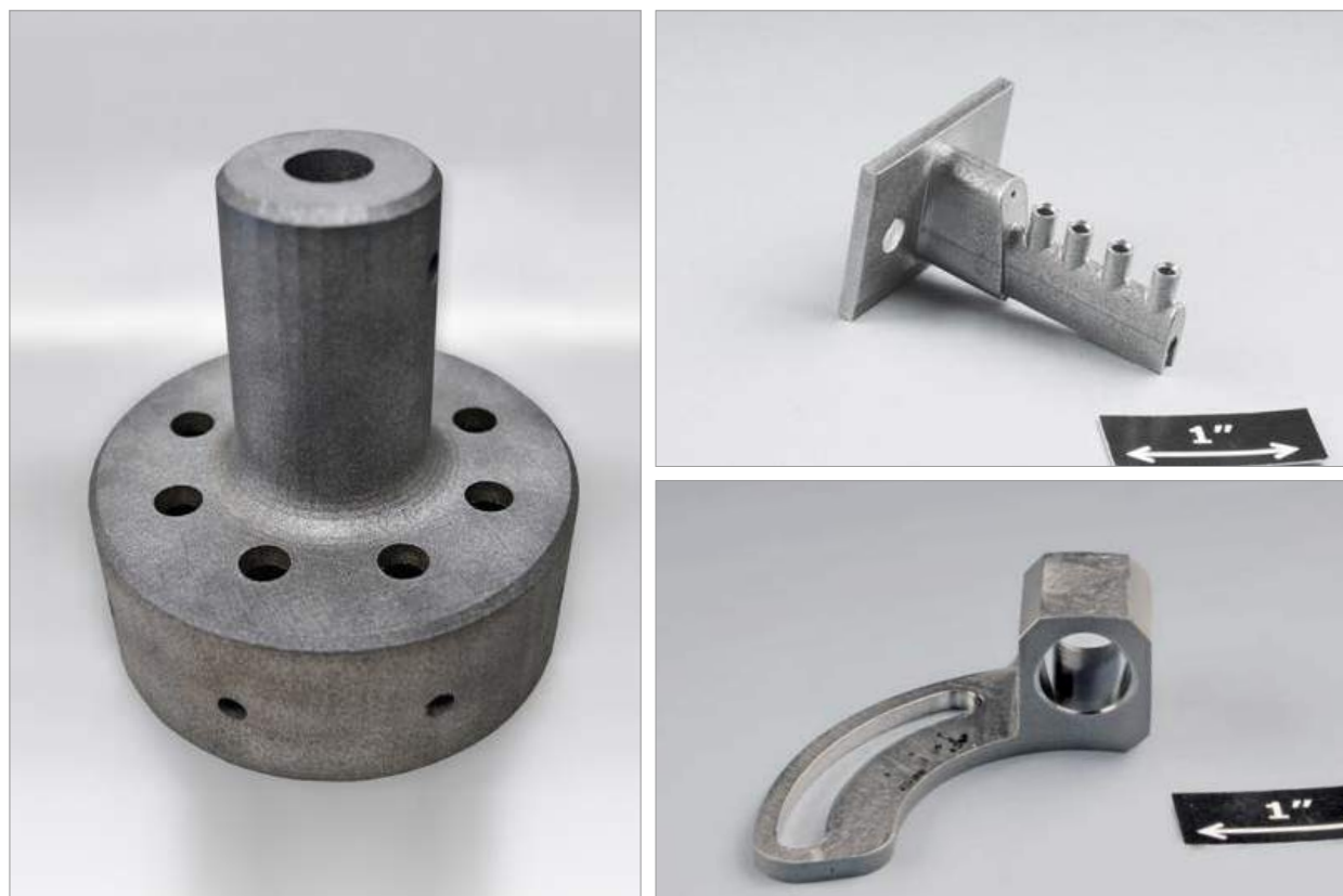
Fig. 6 Some examples of the metal AM tooling currently in use at Honeywell. Left: Carousel for burner rig; top right: Test rake; bottom right, Clamp bracket.
