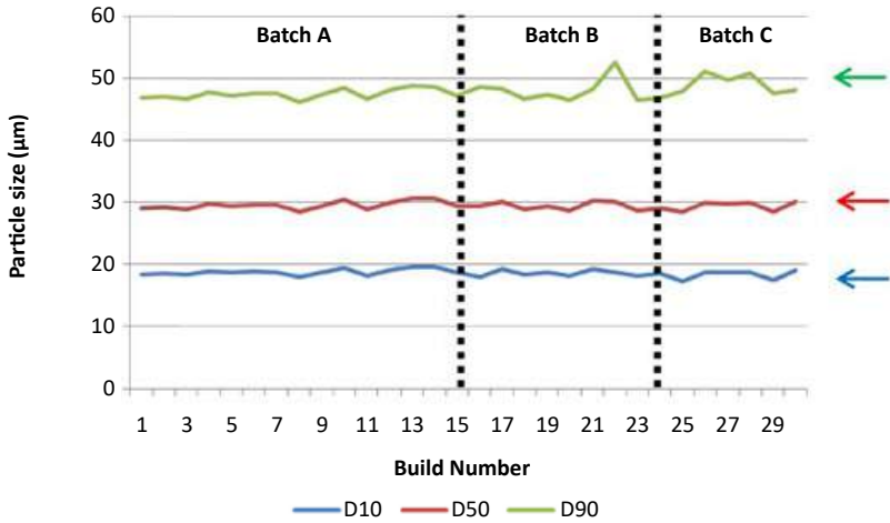
Fig. 11 Variation in particle size – Position 1 [2]
