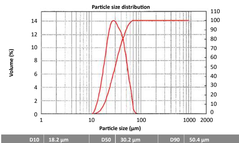
Fig. 9 Particle size distribution data for the original virgin powder [2]
