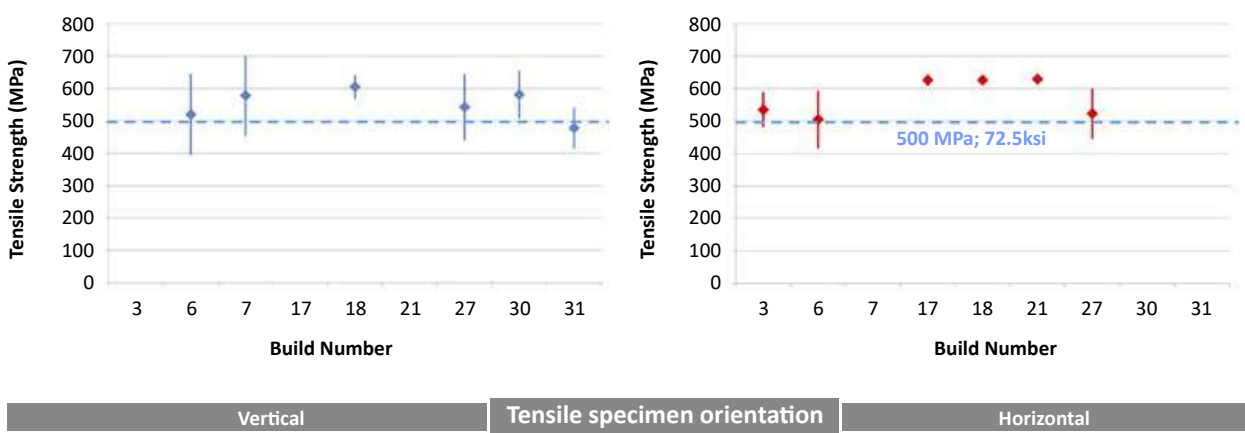
Fig. 15 Tensile strength data throughout the build series [2]
