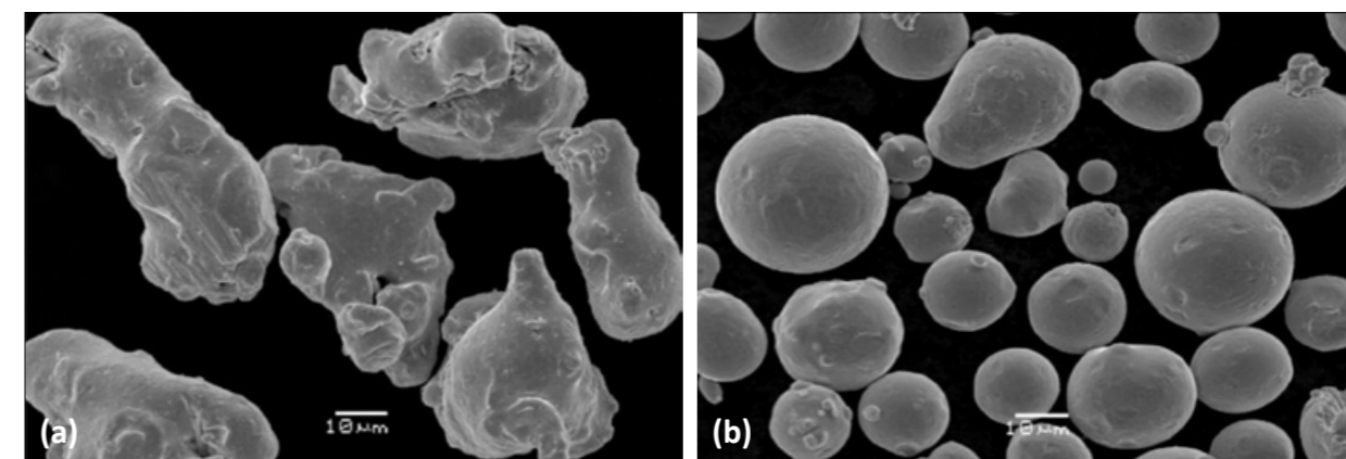
Fig. 4 Morphology of (a) water atomised 316L and (b) gas atomised 316L powder [2]
