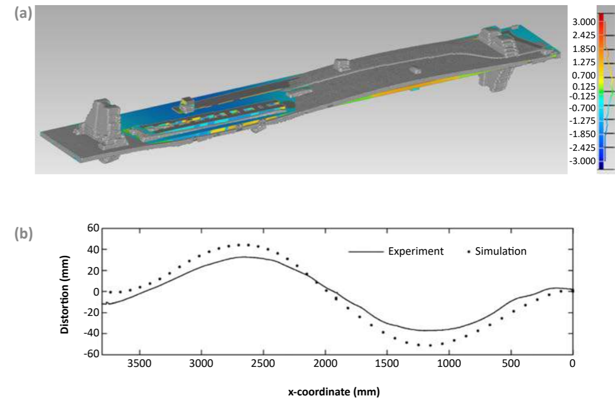
Fig. 8 DED validation study: (a) Sciaky test geometry, (b) simulated vs. experimental distortion of the DED test geometry
