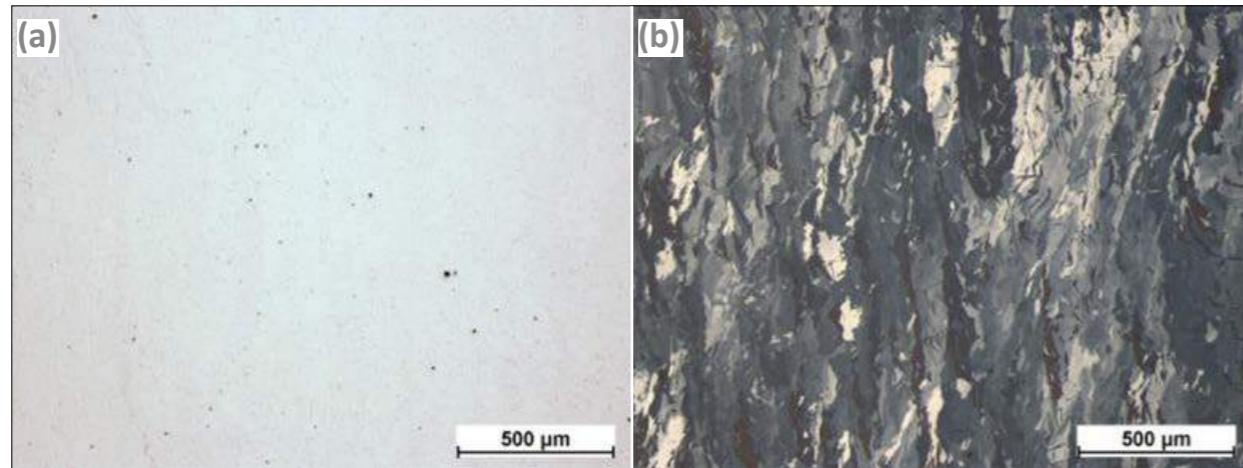
Fig. 18(a) Metallographic analysis shows that a relative density of >99.70% was obtained. (b) Grain growth is mainly parallel to the building direction. Grains grow across multiple layers [3]
