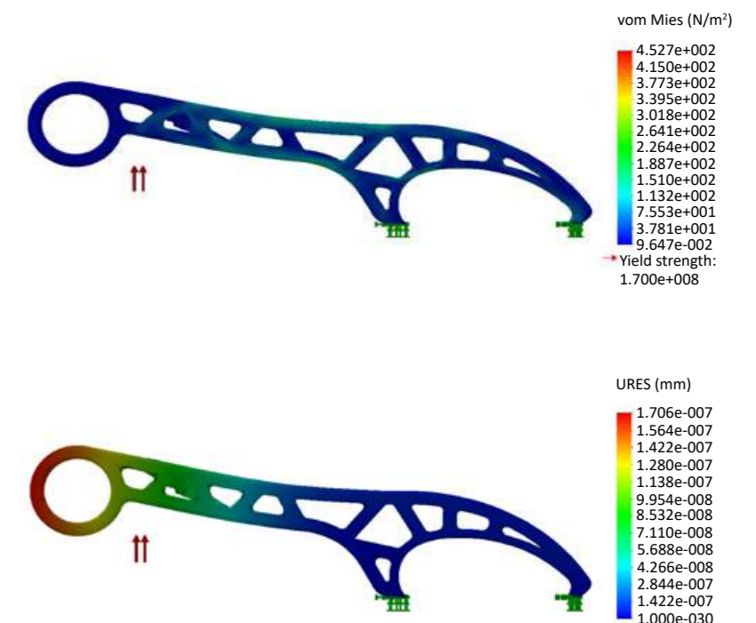
Fig. 5 Stress and displacement analysis of topology optimised bottle opener under 100 N/mm 2 pressure
