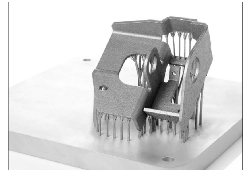
Fig. 4 An example of the use of tree support structures
