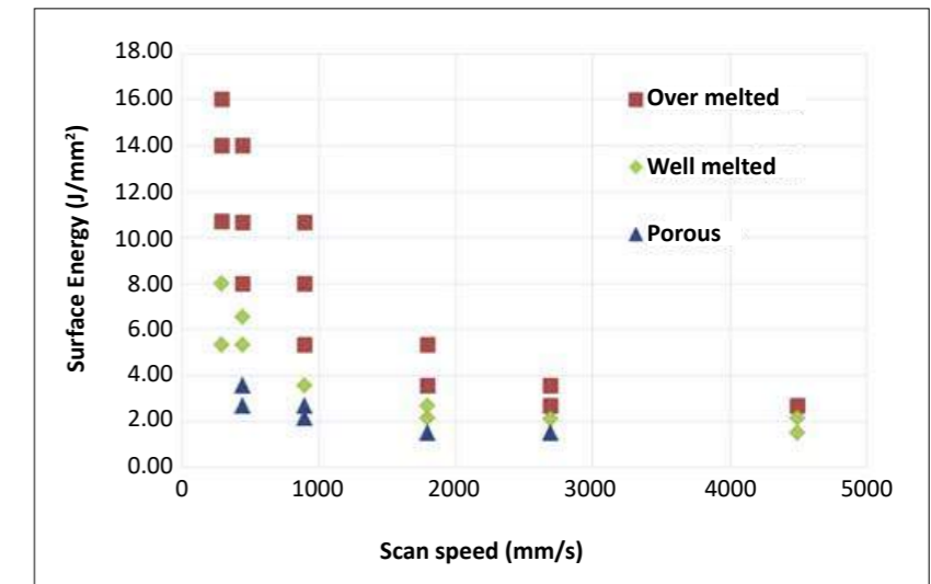
Fig. 5 Process parameter window (in term of Surface Energy and Scan Speed) suitable for well-melted samples [1]
