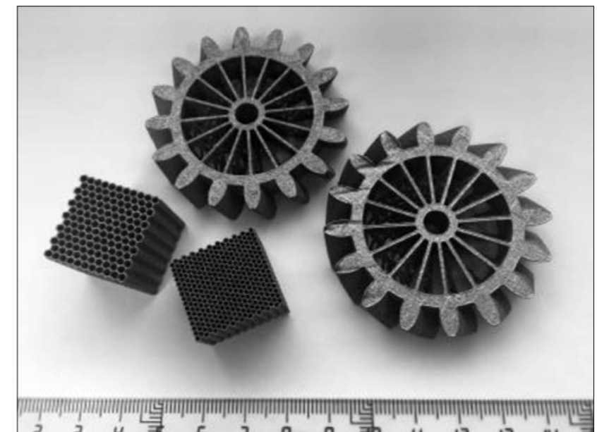
Fig. 13 Prototypes of 316L-6%Cr 3 C 2 processed by SLM [2]
