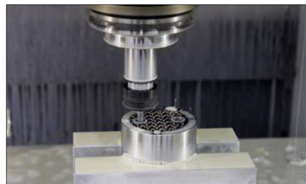
Precision thread milling of special SAE threads on an additively manufactured Inconel component at Imperial's facility in Columbia, New Jersey, USA
