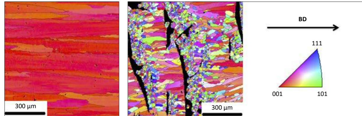
Fig. 6 IPF-map of a well-melted sample (Beam intensity = 5 mA, Scan speed = 900 mm/s and Focus offset = 25 mA) [1]
