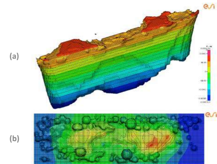
Fig. 2 (a) melted volume along a single track; (b) top view of the same track
