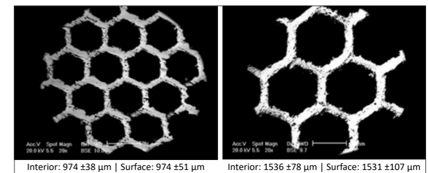
Fig. 14 Details of the cell sizes of two different honeycombs [2]
