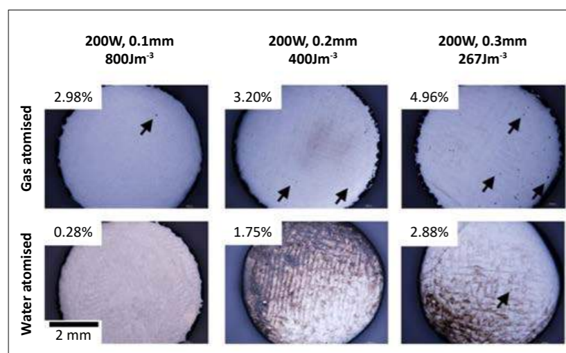
Fig. 2 Optical micrographs of the Co-33Cr-5Mo-0.4N alloy samples built by PBF with the gas and water atomised powders [1]
