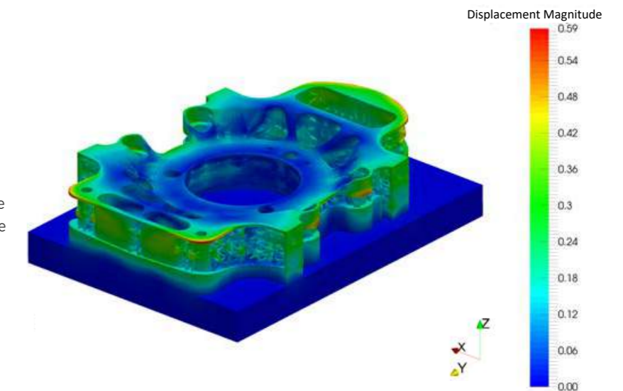
Fig. 1 Sample powder bed fusion simulation part, dimensions are roughly 275 x 200 x 40 mm
