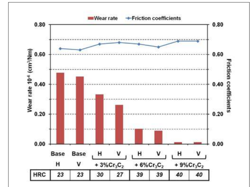
Fig. 12 Wear rates and friction coefficients for the SLM-processed materials [2]
