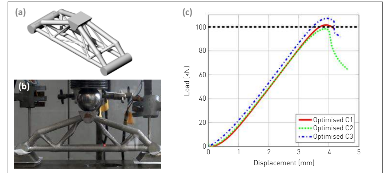
Fig. 4 Simple beam (after Smith et al. 2016): (a) design; (b) fabricated component during a load test, and (c) load vs. displacement responses of tested components (target load = 100 kN)
