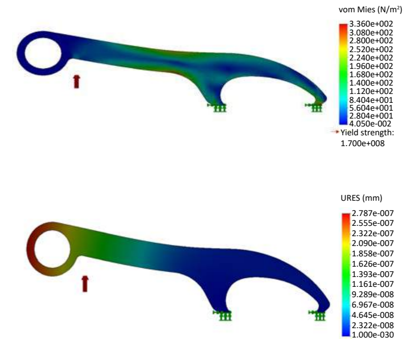
Fig. 4 Stress and displacement analysis of solid bottle opener under 100 N/mm 2 pressure
