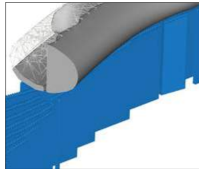
Fig. 11 Additional solid material placed under the lattice
