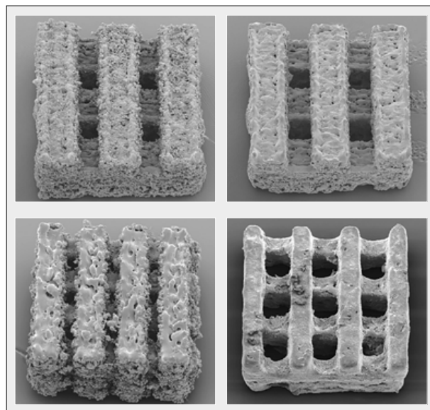
Fig. 12 Magnesium scaffolds approx. 3x3 mm. Top row: MgCa0.8, bottom row: WE43 alloy. Left: as-printed, right: after secondary treatment in aqueous nitric acid (SEM Courtesy Laser Zentrum Hannover)
