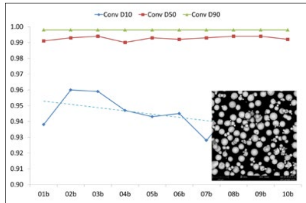
Fig. 18 Decreasing convexity of Ti-6Al-4V powder lots through repeated re-uses [5]
