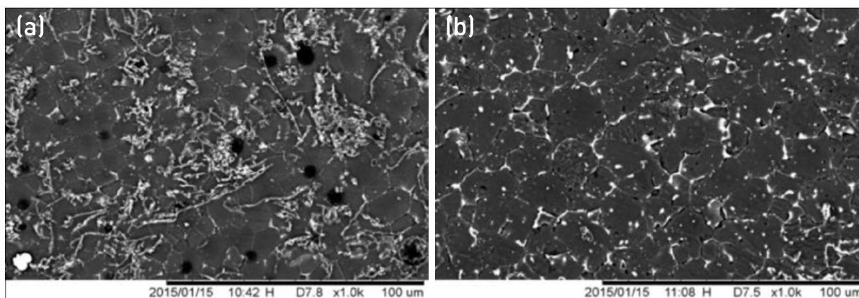
Fig. 8 SEM micrographs showing (a) "skin clusters" in as-deposited sample and (b) fully dense microstructure of a HIPed sample [2]
