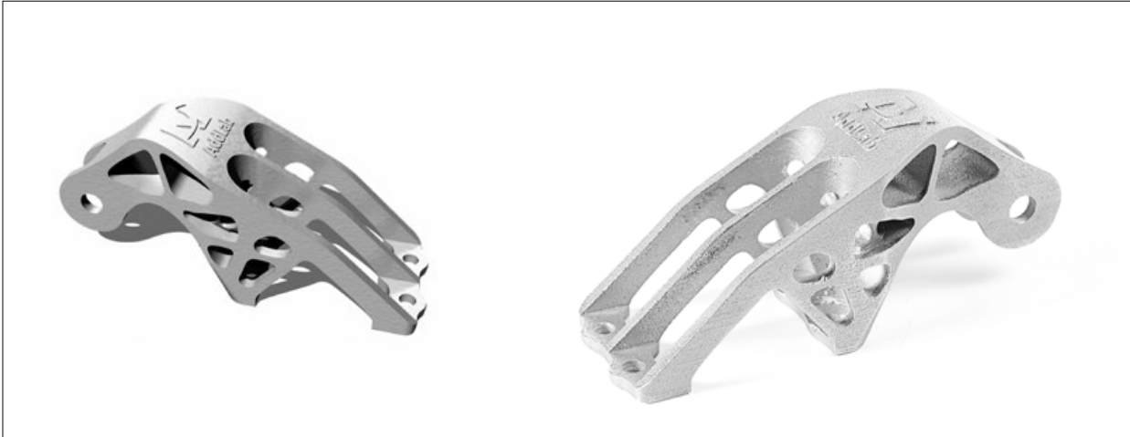
Fig. 5 Computer designed AM part (left) and manufactured part (right) (Courtesy Additive Industries/AddLab)
