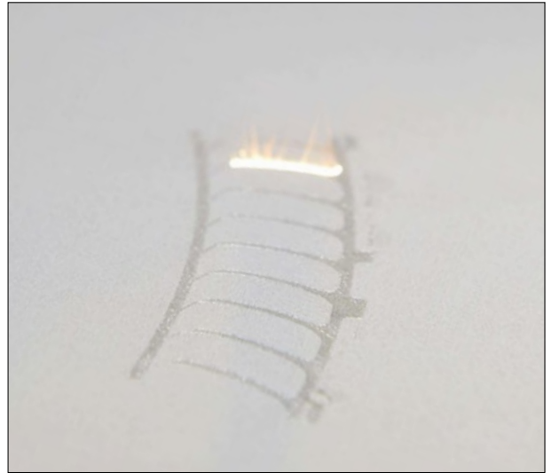
Fig. 6 Additive Manufacturing of a vane cluster at MTU in Munich (Courtesy MTU Aero Engines)
