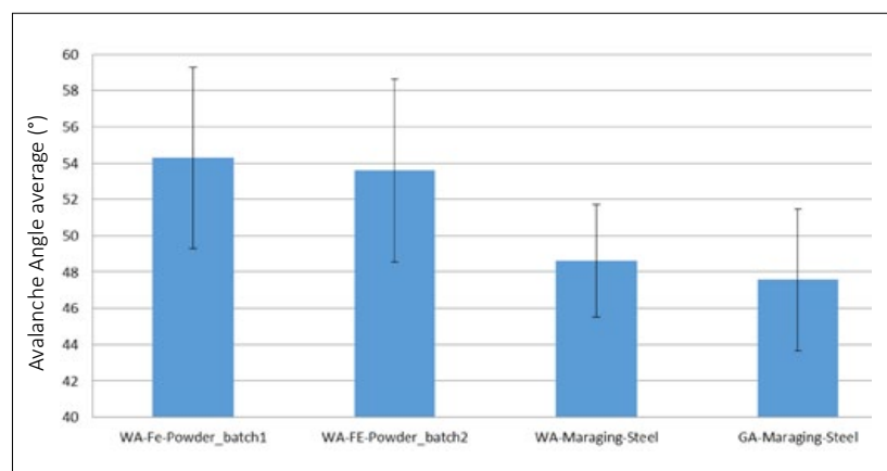
Fig. 10 Average avalanche angle of analysed powders [3]
