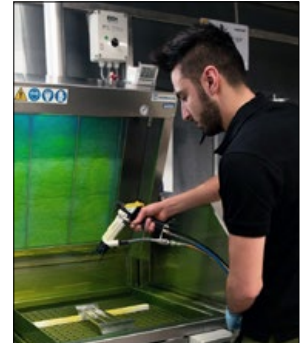
Components are wetted with a fluorescent penetrant
