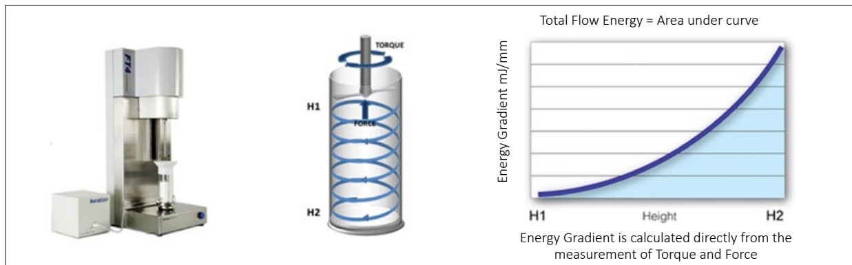
Fig. 12 Measurement of flow energy using the FT4 Powder Rheometer® [4]
