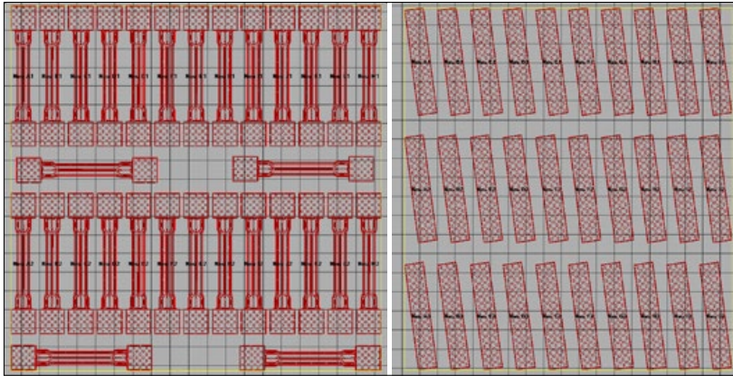
Fig. 11 Overview of build jobs for 30 specimens for tensile test (left) and Charpy V-notch test (right) [3]
