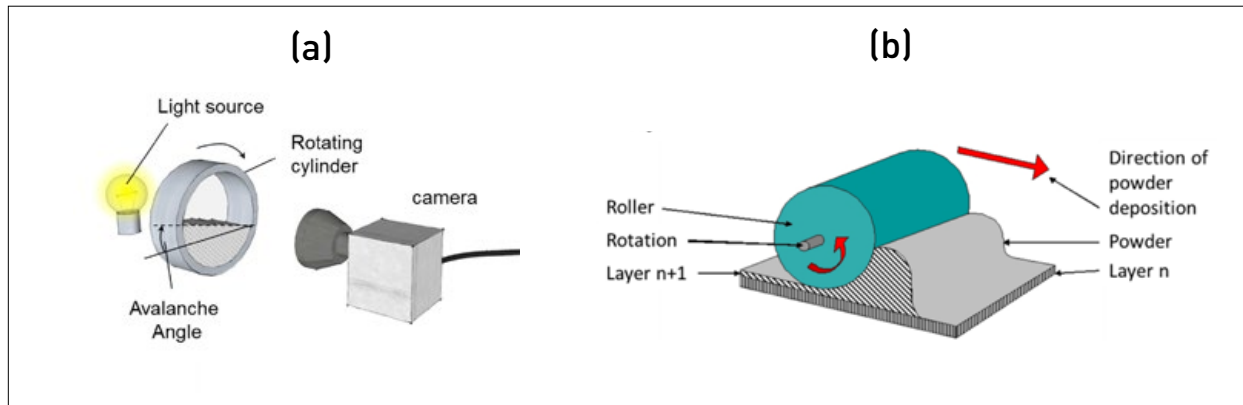
Fig. 9 Schematic of the (a) Revolution Powder Analyser © Mercury Scientific Inc (b) powder deposition process during Additive Manufacturing [3]
