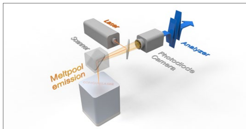
Fig. 1 In-situ monitoring of the melt pool with QMmeltpool 3D: A photo diode and a camera provide coaxial monitoring of the area and intensity of the melt pool through the laser optic with exact positioning
