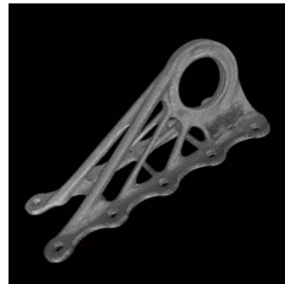
Fig. 5b QMmeltpool 3D display of the cabin bracket from the Airbus A350 XWB with reduced laser output
