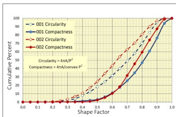
Fig. 23 The results of circularity and compactness testing of gas atomised 316L powder samples 001 and 002. The results are shown as cumulative plots of the frequency distributions [6]
