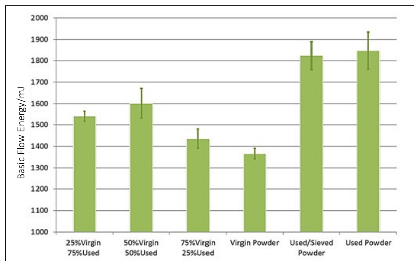
Fig. 13 Using powder rheology to optimise the use of recycled materials [4]
