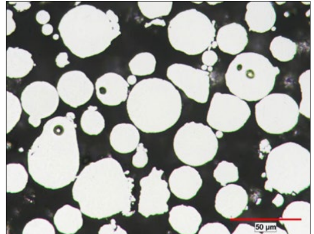
Fig. 21 Cross-sections of a maraging steel powder metallographically prepared and imaged (unetched) [6]
